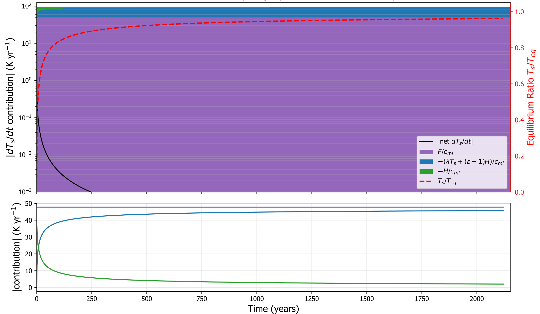
CCSM3: surface tendency budget ( \kappa=3.9\text{e-}05 , h_{ml}=1 m, \varepsilon=0.89 )
