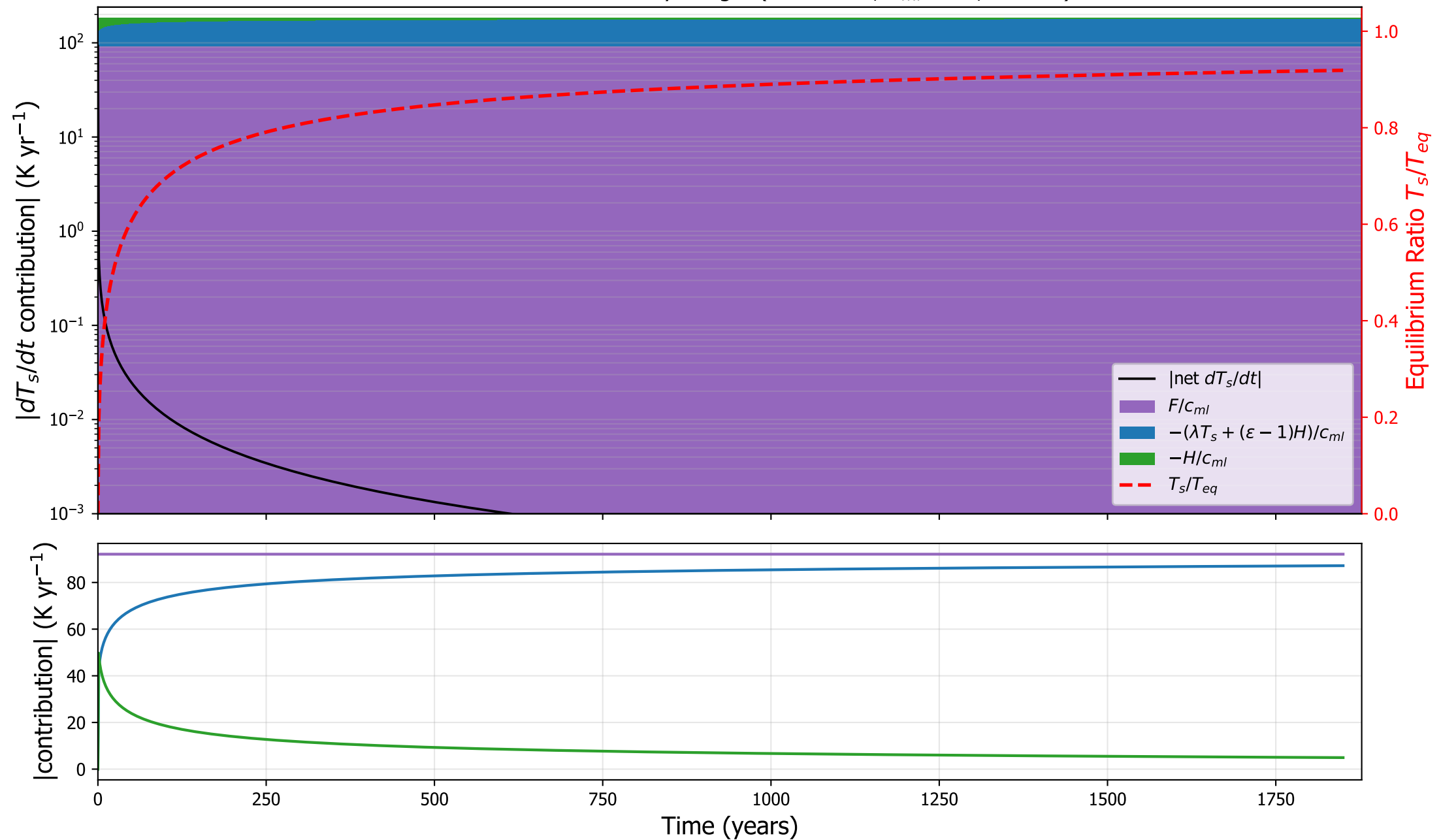
CNRMCM6: surface tendency budget ( \kappa=5.3\text{e-}05 , h_{ml}=1 m, \varepsilon=1.51 )
