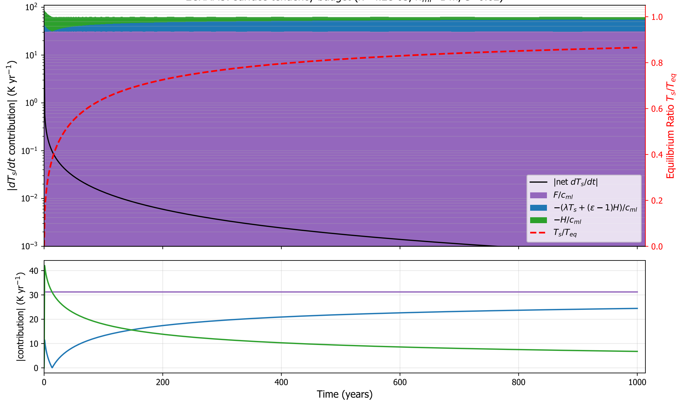
ECHAM5: surface tendency budget ( \kappa=4.2\text{e-}05 , h_{ml}=1 m, \varepsilon=0.62 )
