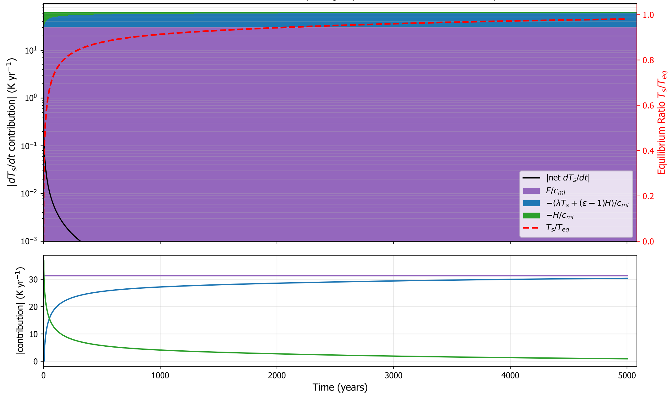
GISSE2R: surface tendency budget ( \kappa=8.4\text{e-}05 , h_{ml}=1 m, \varepsilon=0.66 )
