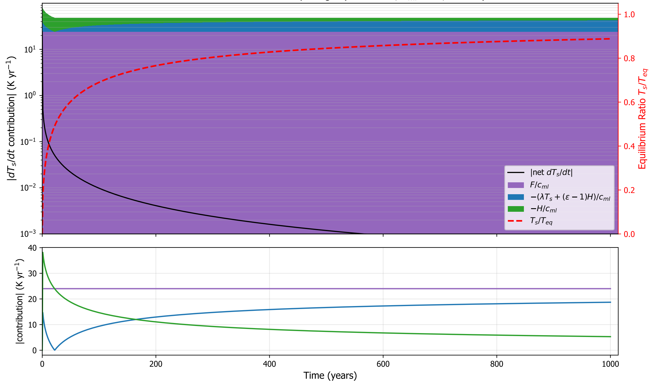
IPSLCM5A: surface tendency budget ( \kappa=4.3\text{e-}05 , h_{ml}=1 m, \varepsilon=0.51 )
