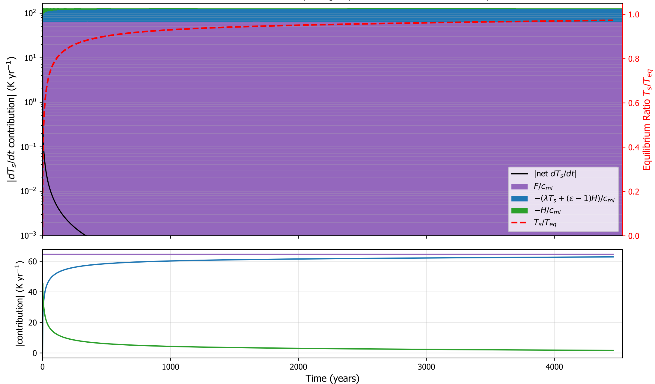
MPIESM11: surface tendency budget ( \kappa=5.2\text{e-}05 , h_{ml}=1 m, \varepsilon=1.04 )
