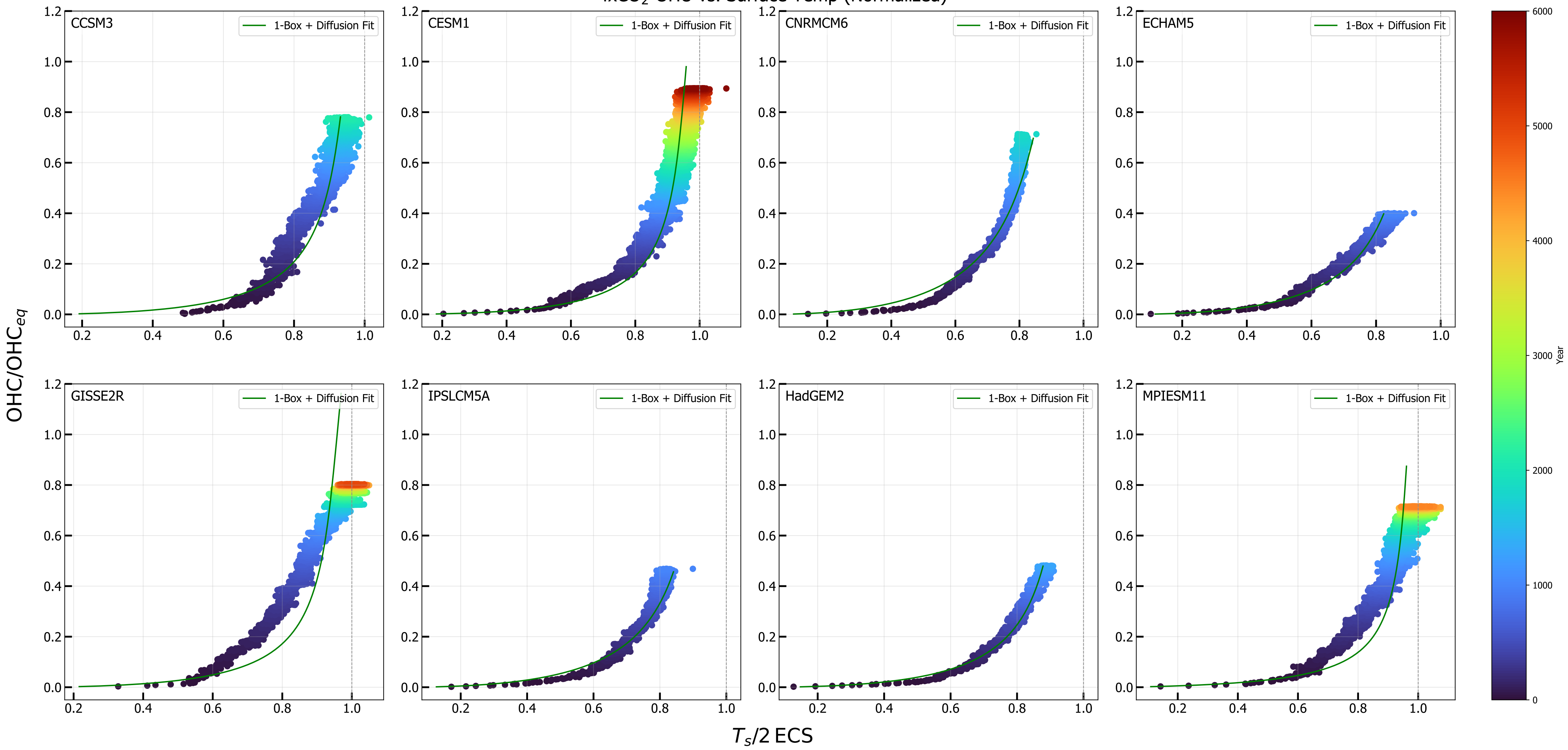
4xCO 2 OHU vs. Surface Temp (Normalized)
