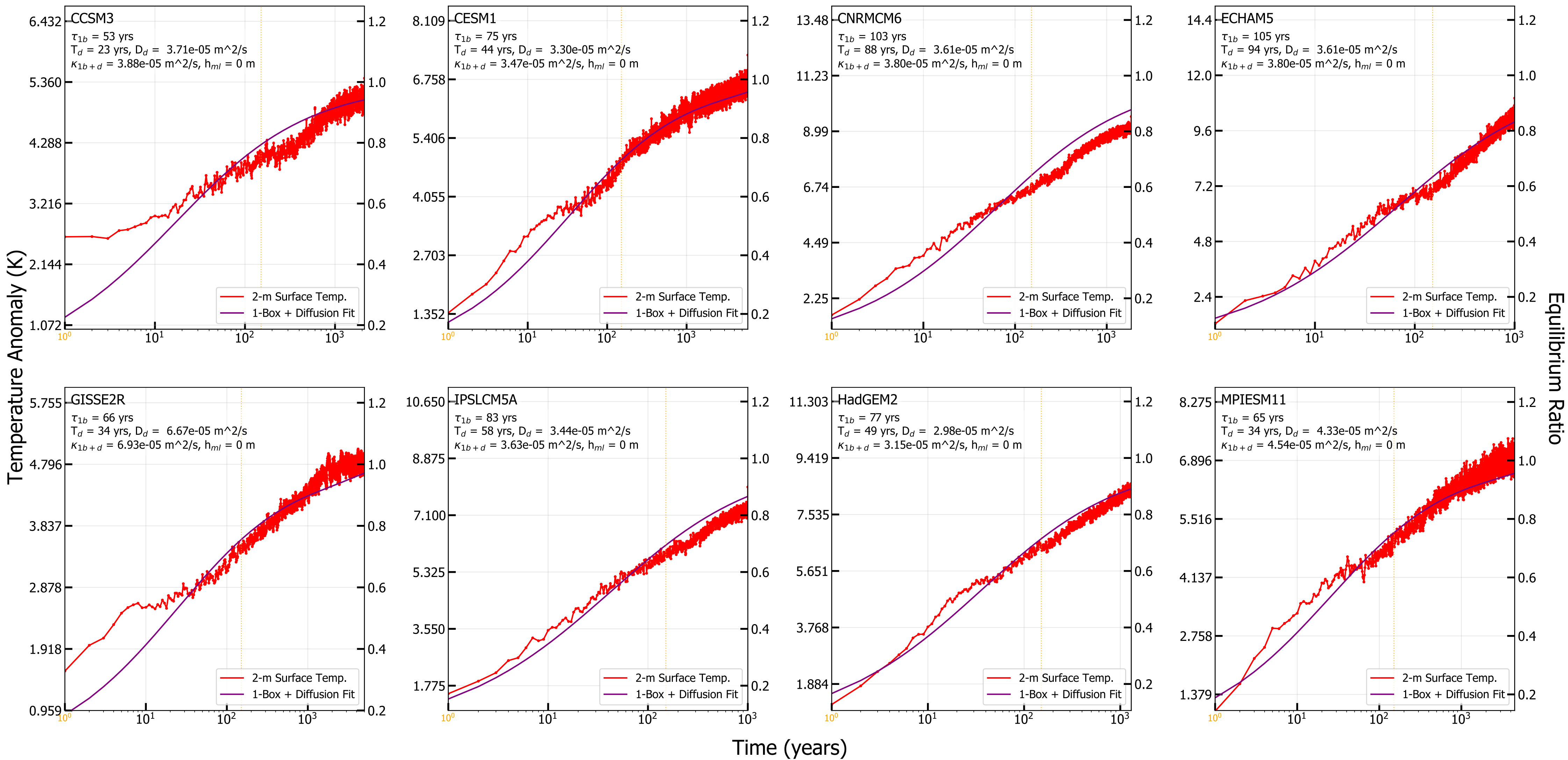
4xCO 2 T 2M vs. Time w/ Diffusive Fit
