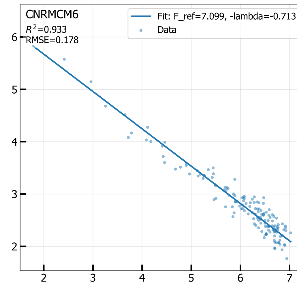
4xCO 2 Net TOA vs T 2M
