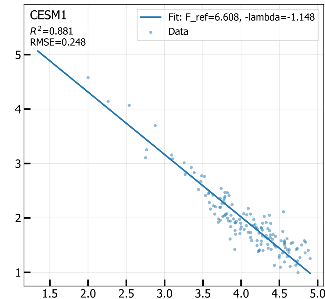
4xCO 2 Net TOA vs T 2M
