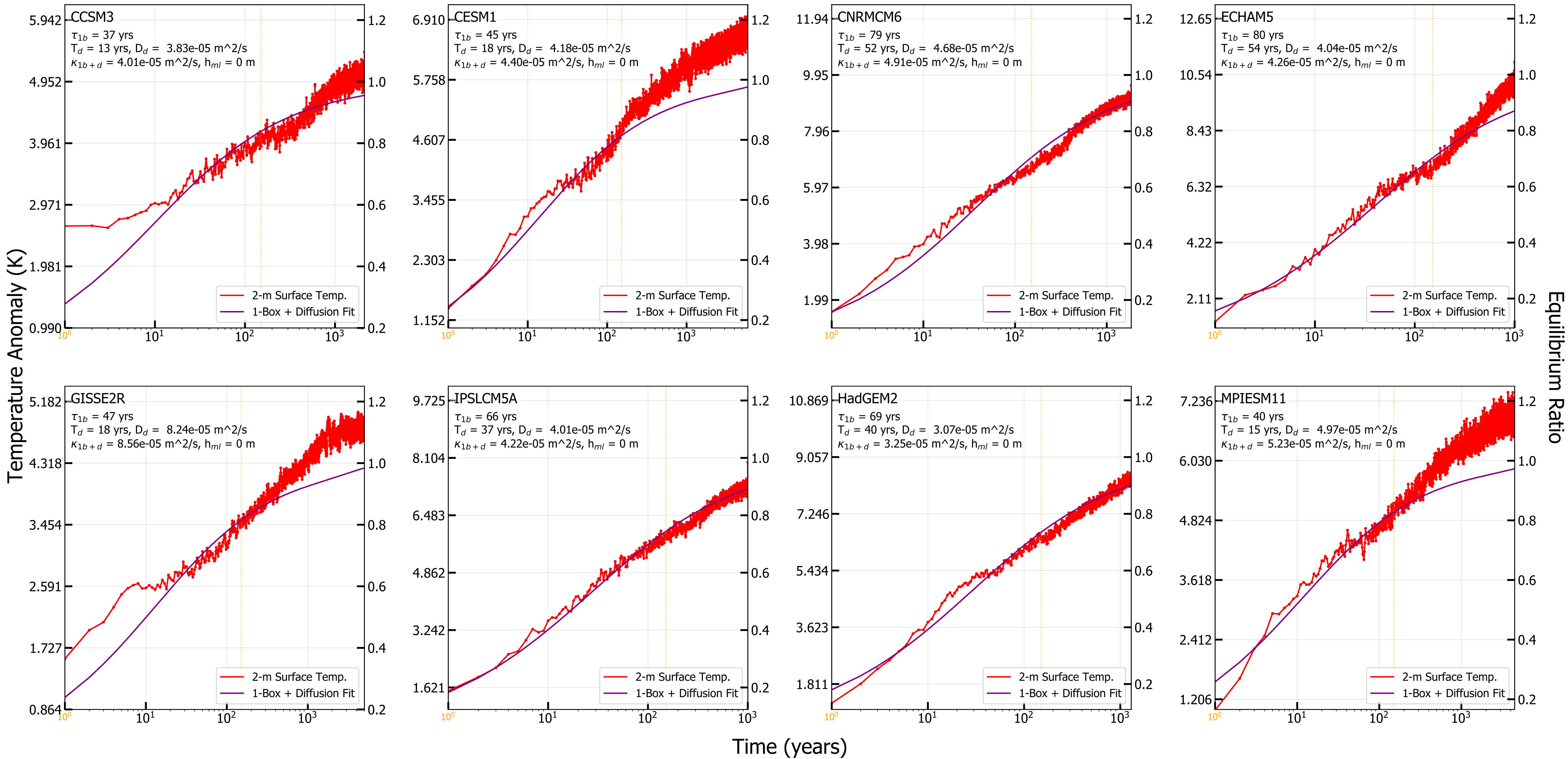
4xCO 2 T 2M vs. Time w/ Diffusive Fit
