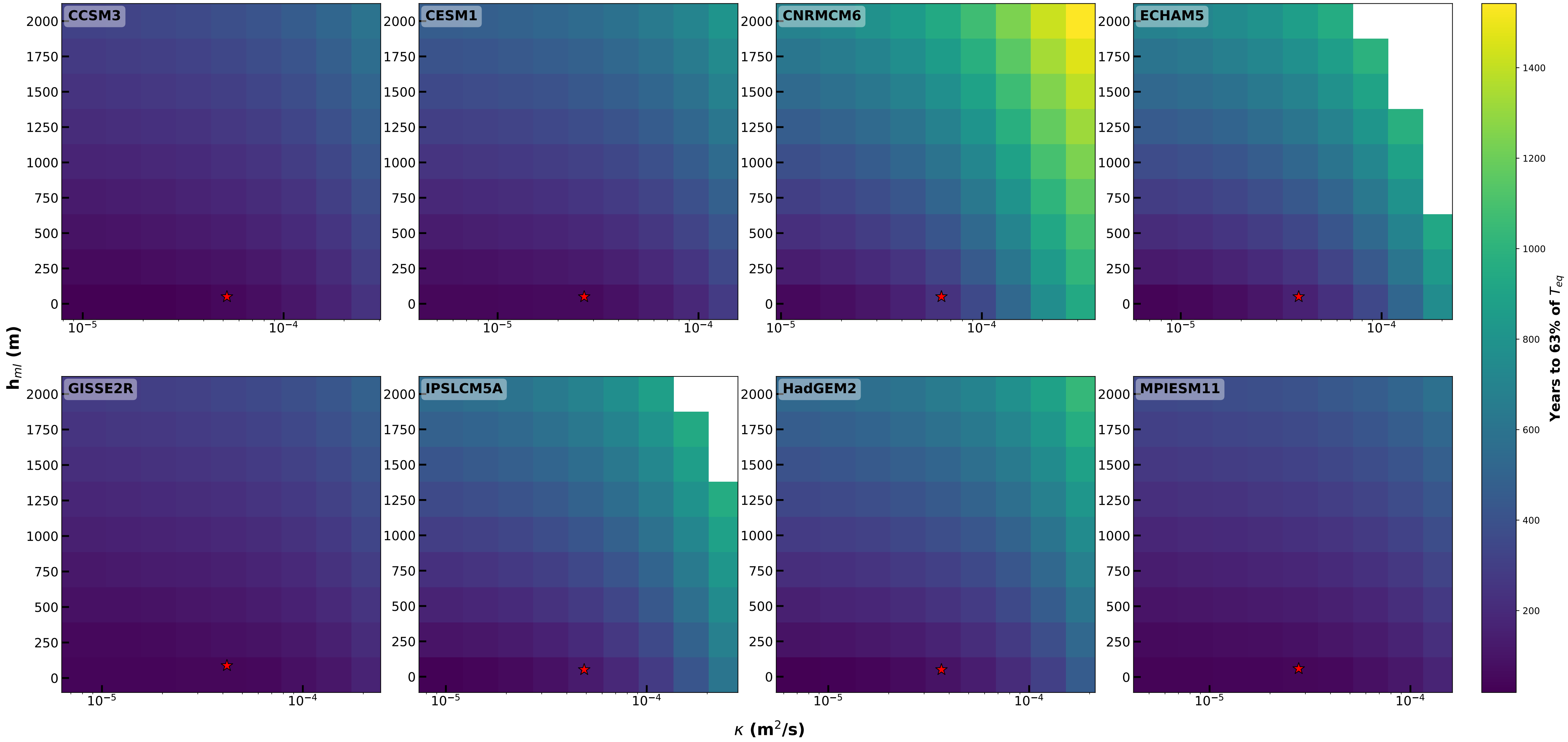
Years to Reach 63% of T_{eq} vs. K/h_{ml}
