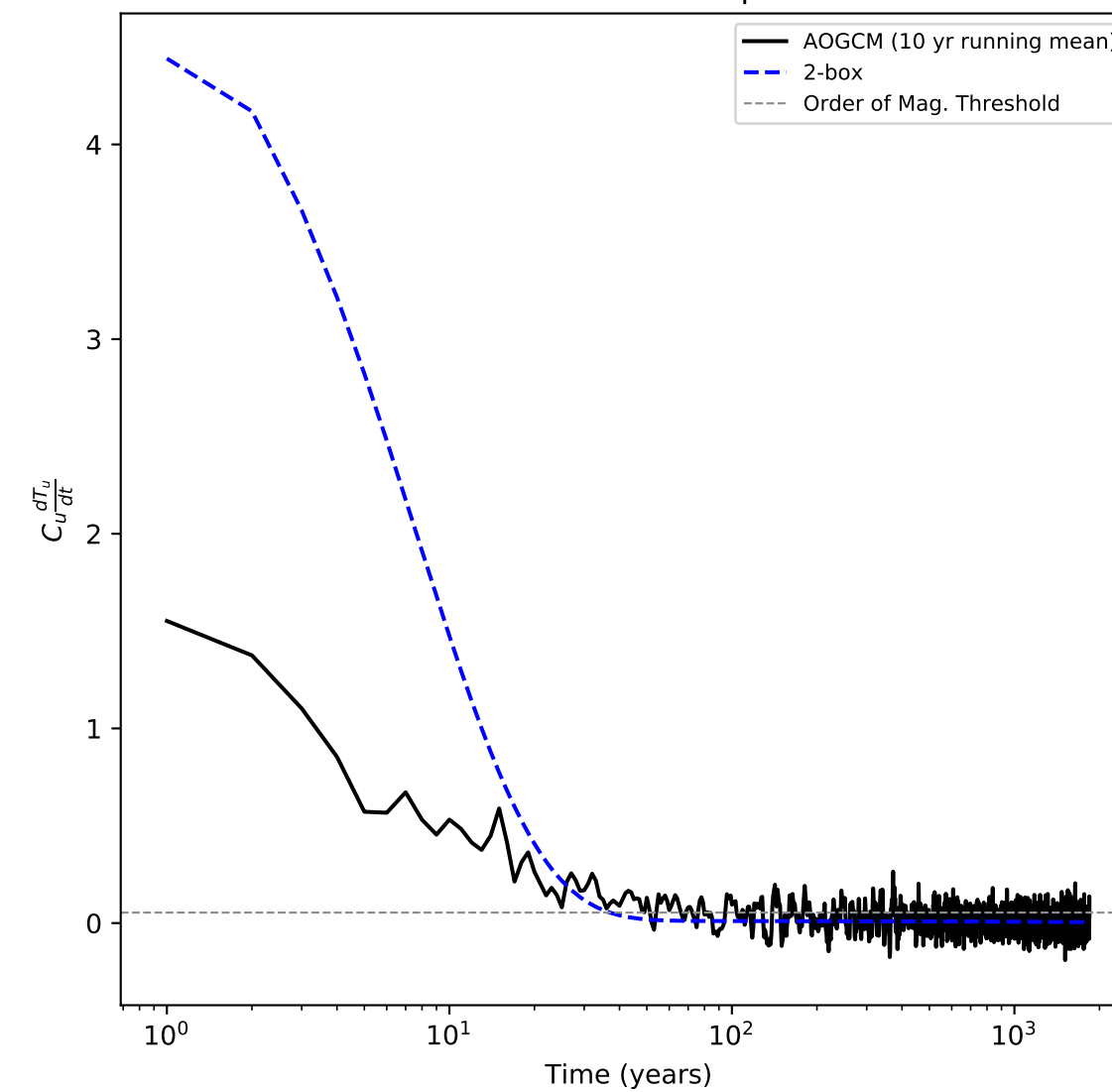
HadGEM2 4xCO2: Assumption 2 Test
