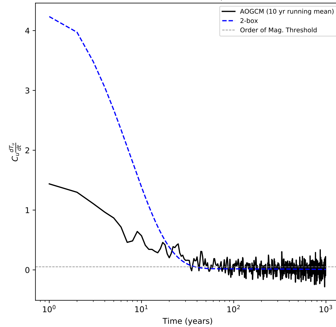
IPSLCM5A 4xCO2: Assumption 2 Test
