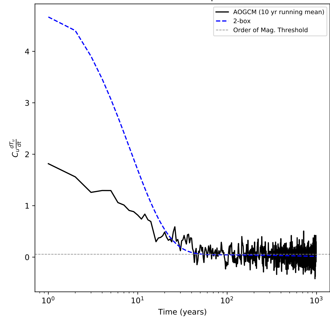
MPIESM11 4xCO2: Assumption 2 Test
