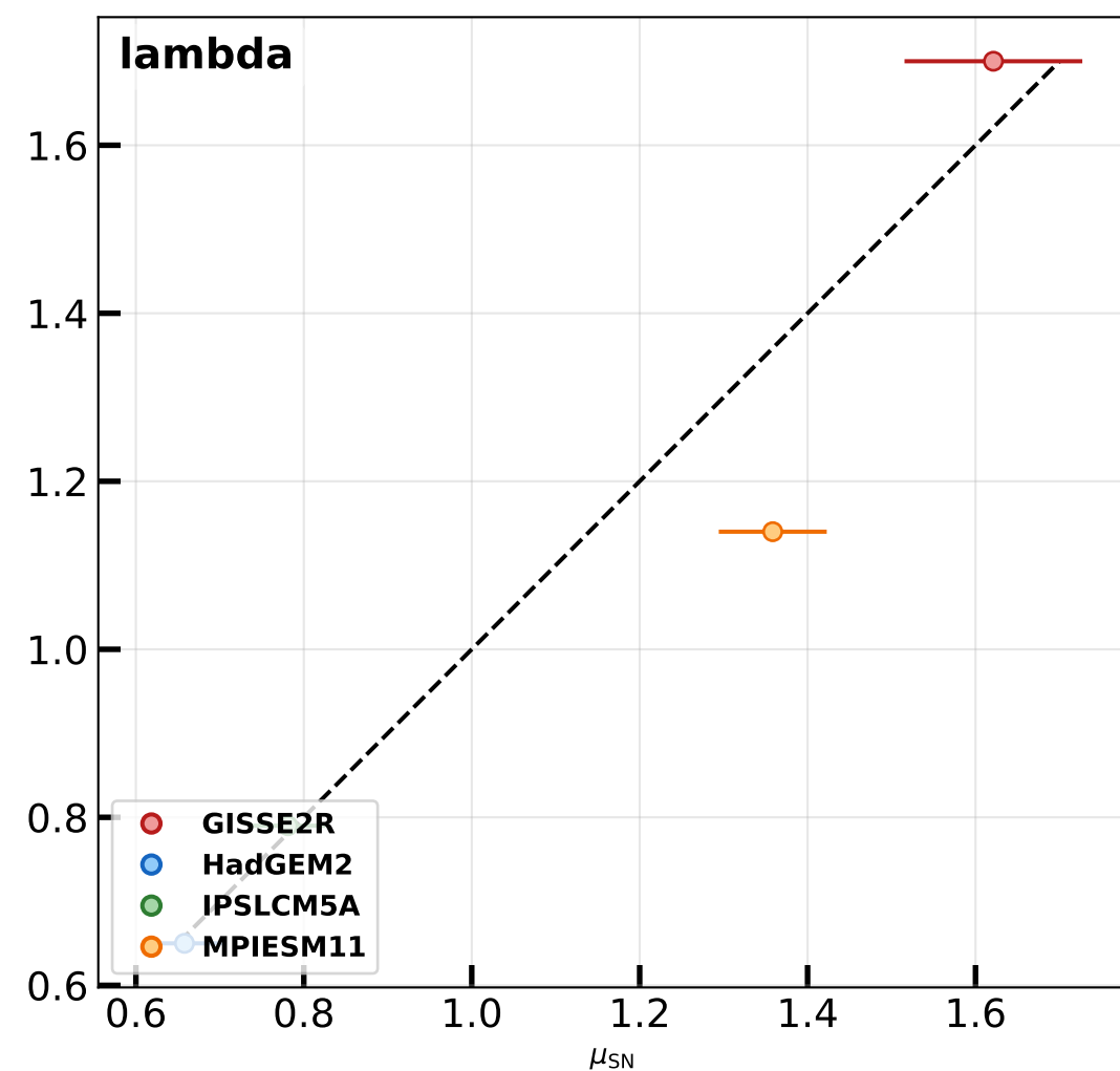
4xCO2 Geoffroy vs. Sanjit/Nadir (w/ 95% CI)
