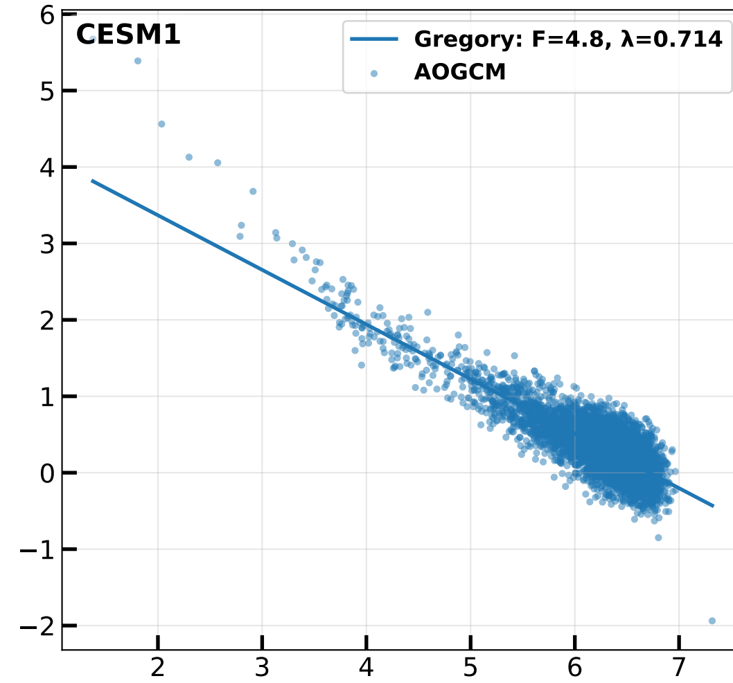
4xCO 2 Net TOA vs T 2M (radiative fit, iter 1)
