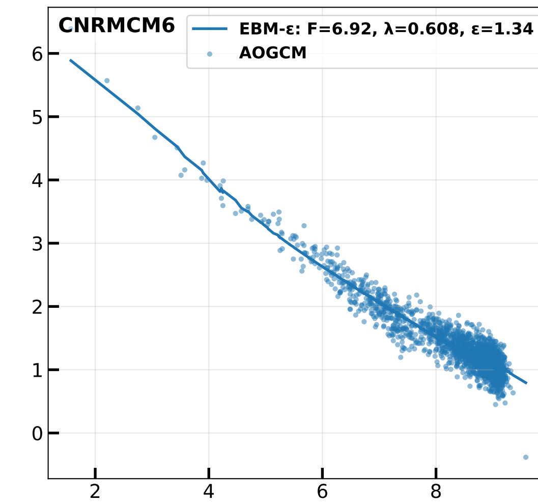
4xCO 2 Net TOA vs T 2M (radiative fit, iter 5)
