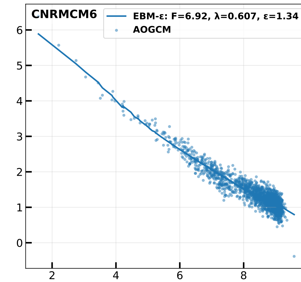
4xCO 2 Net TOA vs T 2M (radiative fit, iter 6)
