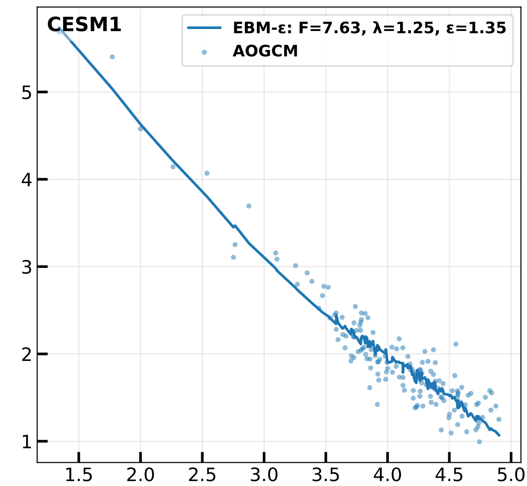
4xCO 2 Net TOA vs T 2M (radiative fit, iter 6)
