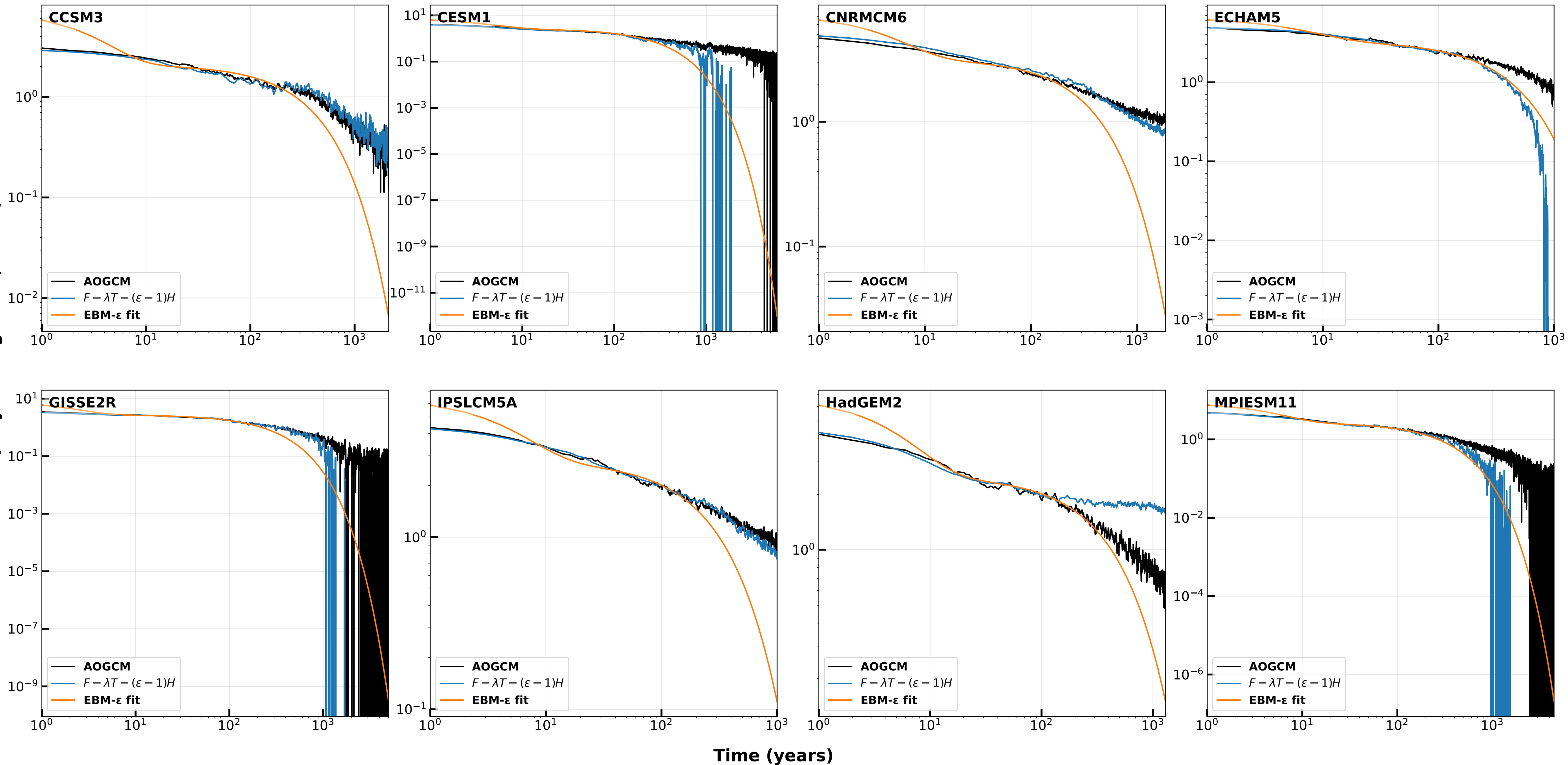
4xCO 2 Net TOA vs. Time
