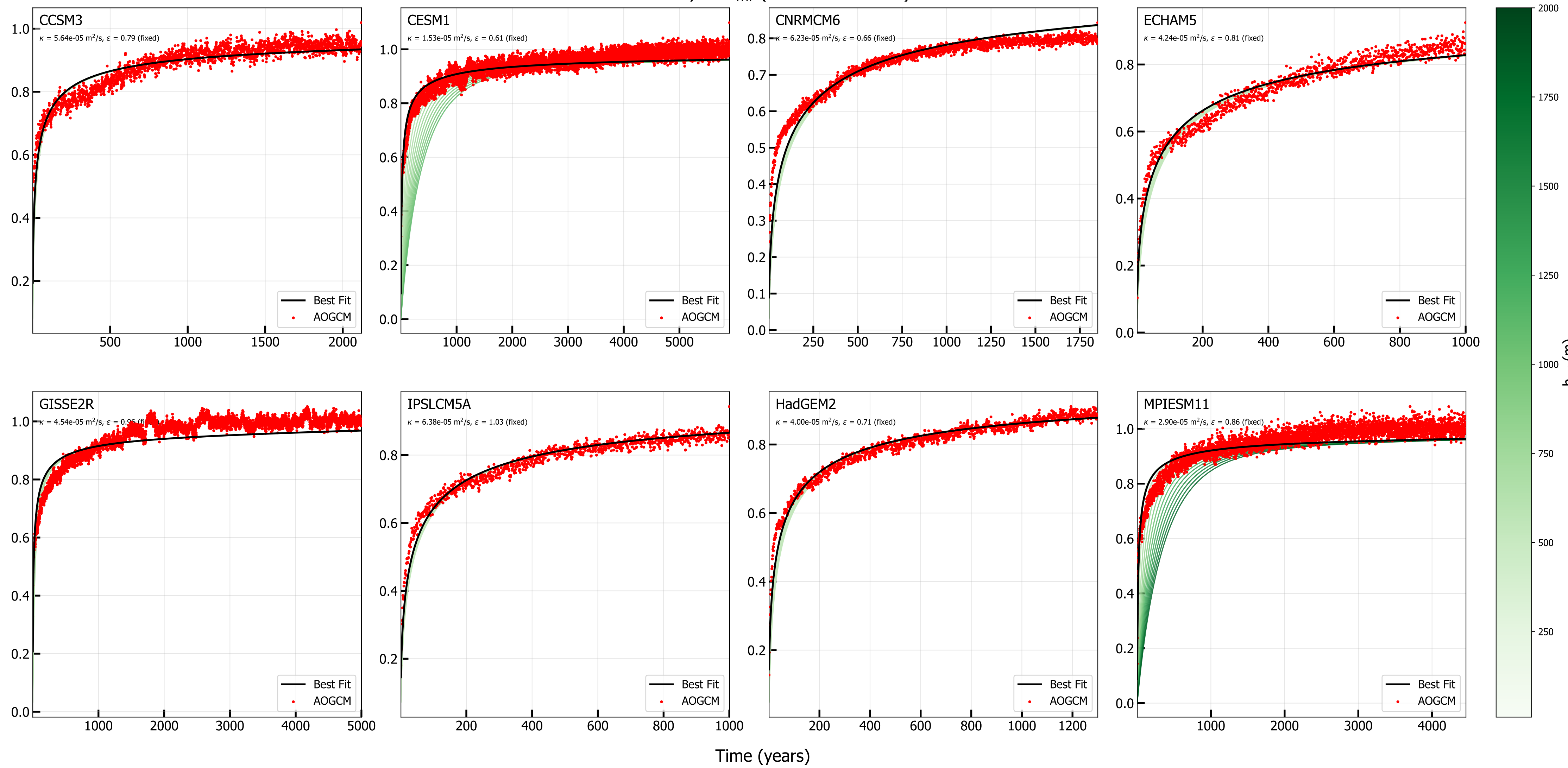
Sensitivity to h_{ml} ( \kappa held at best fit)
