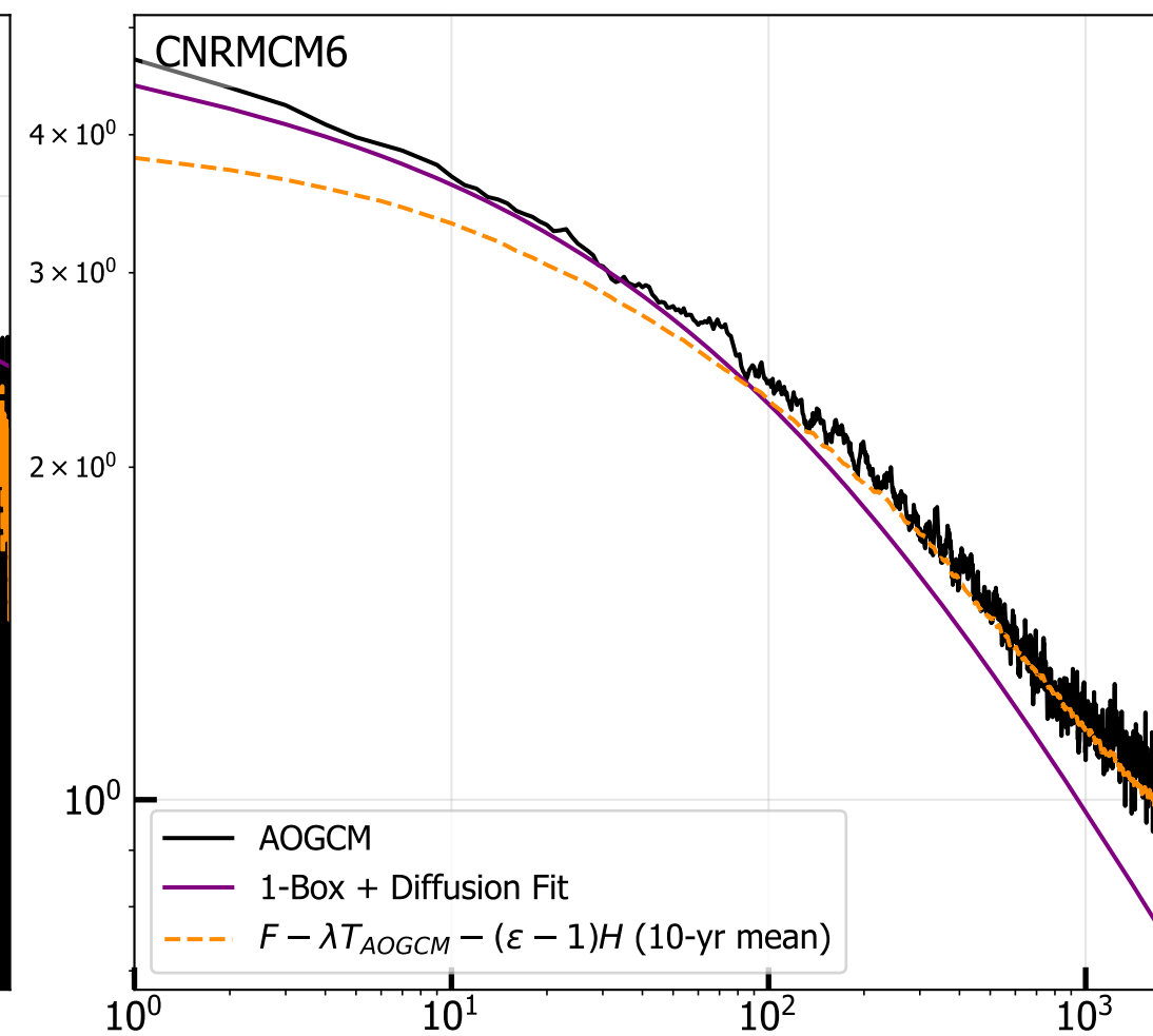
4xCO 2 Net TOA vs. Time
