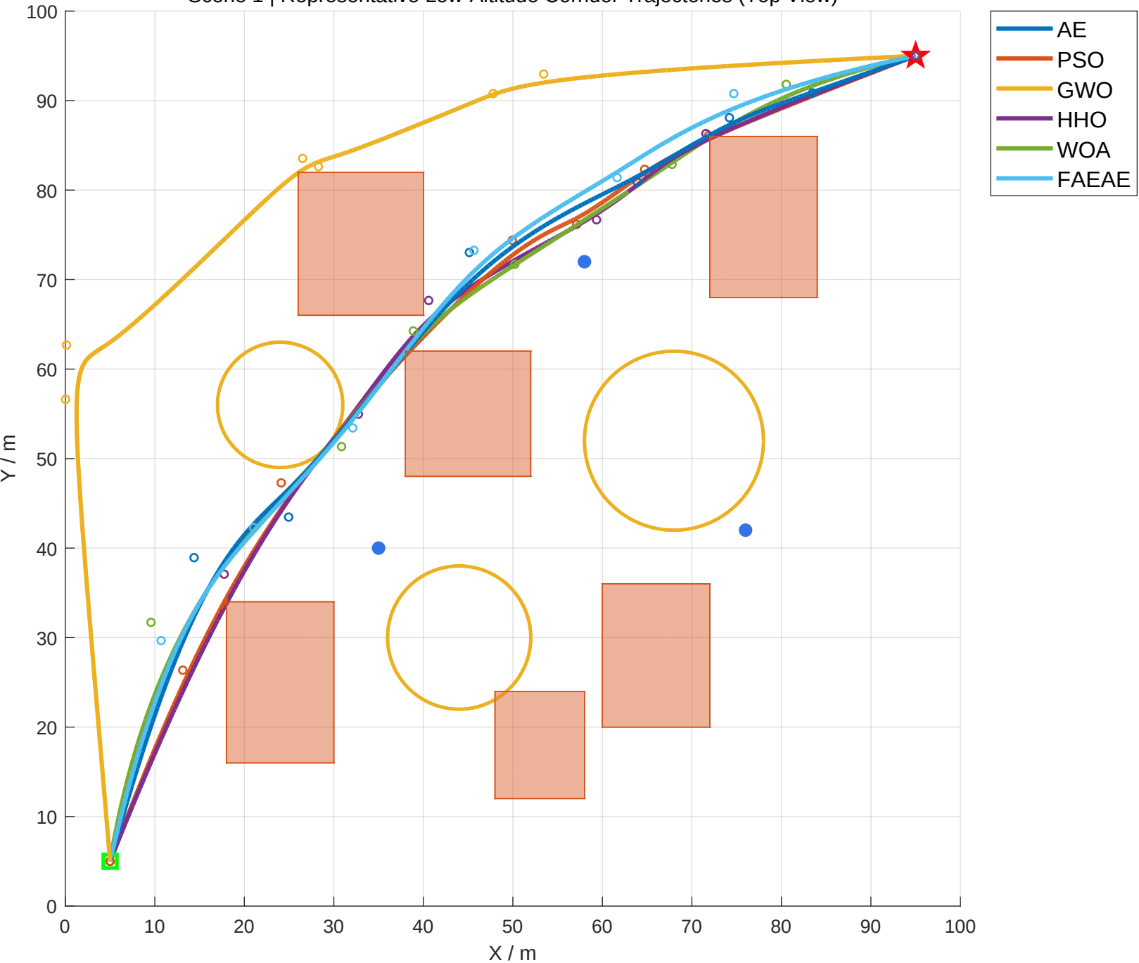
Scene 1 | Representative Low-Altitude Corridor Trajectories (Top View)
