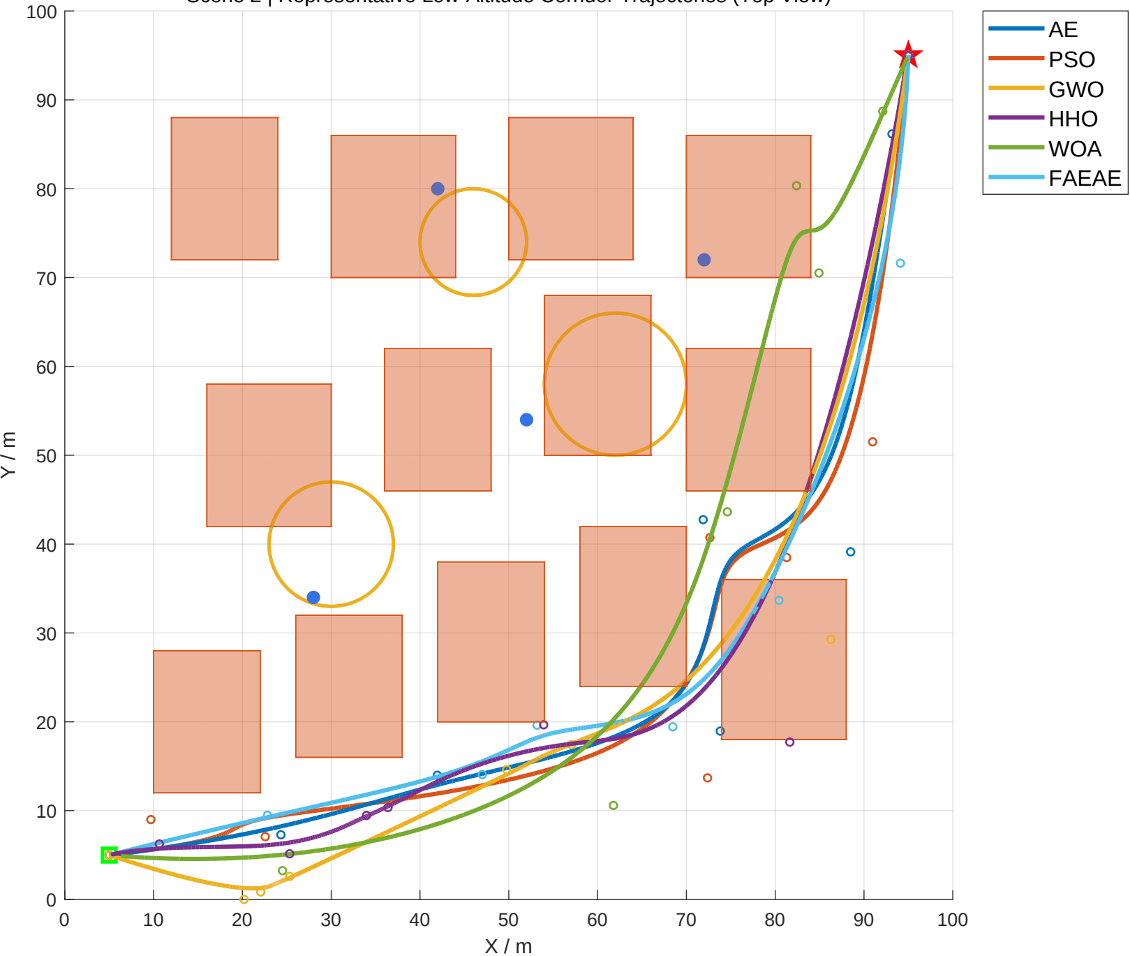
Scene 2 | Representative Low-Altitude Corridor Trajectories (Top View)
