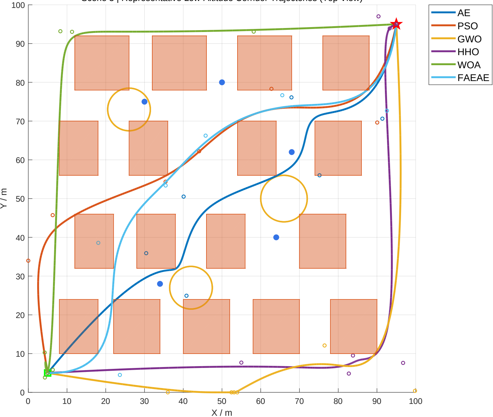
Scene 3 | Representative Low-Altitude Corridor Trajectories (Top View)
