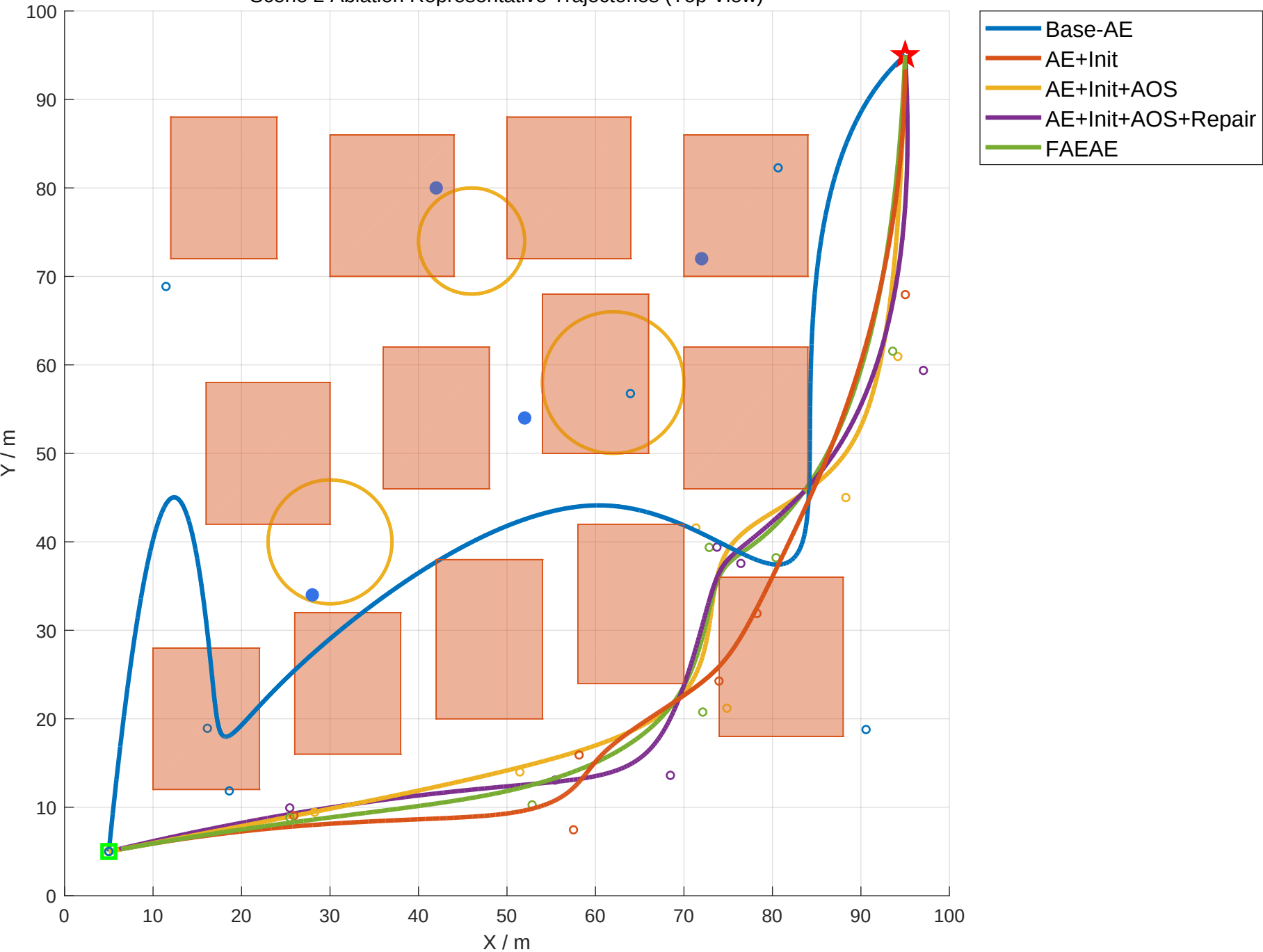
Scene 2 Ablation Representative Trajectories (Top View)
