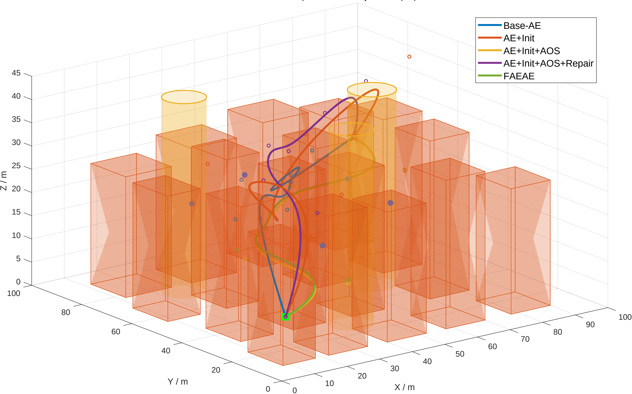
Scene 3 Ablation Representative Trajectories (3D)
