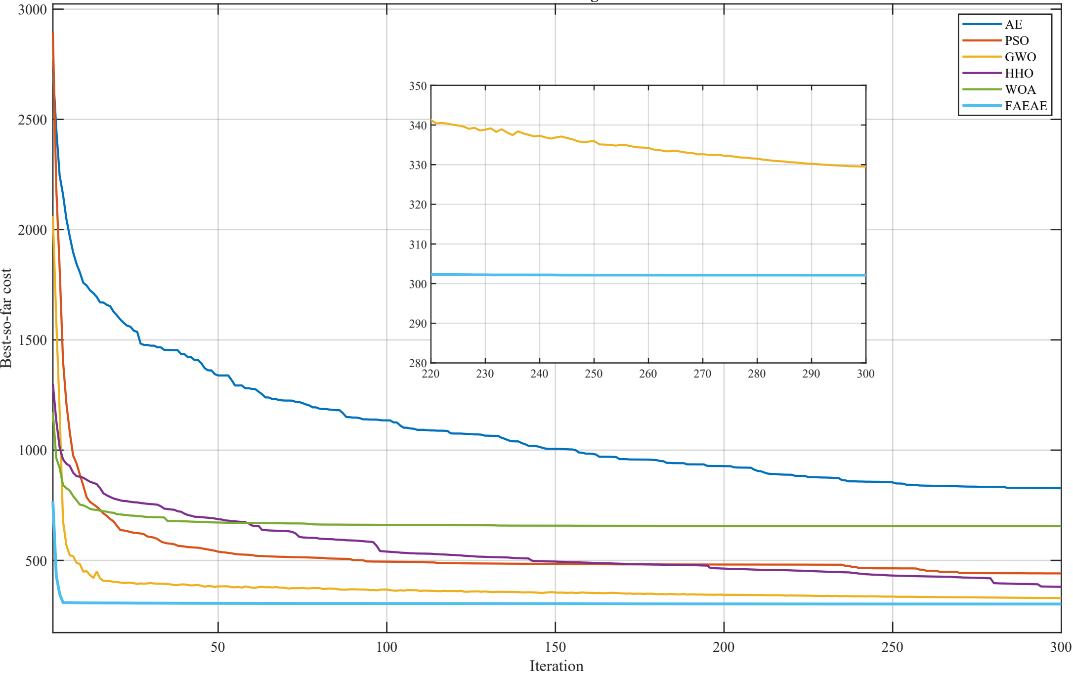
Scene 1 Convergence
