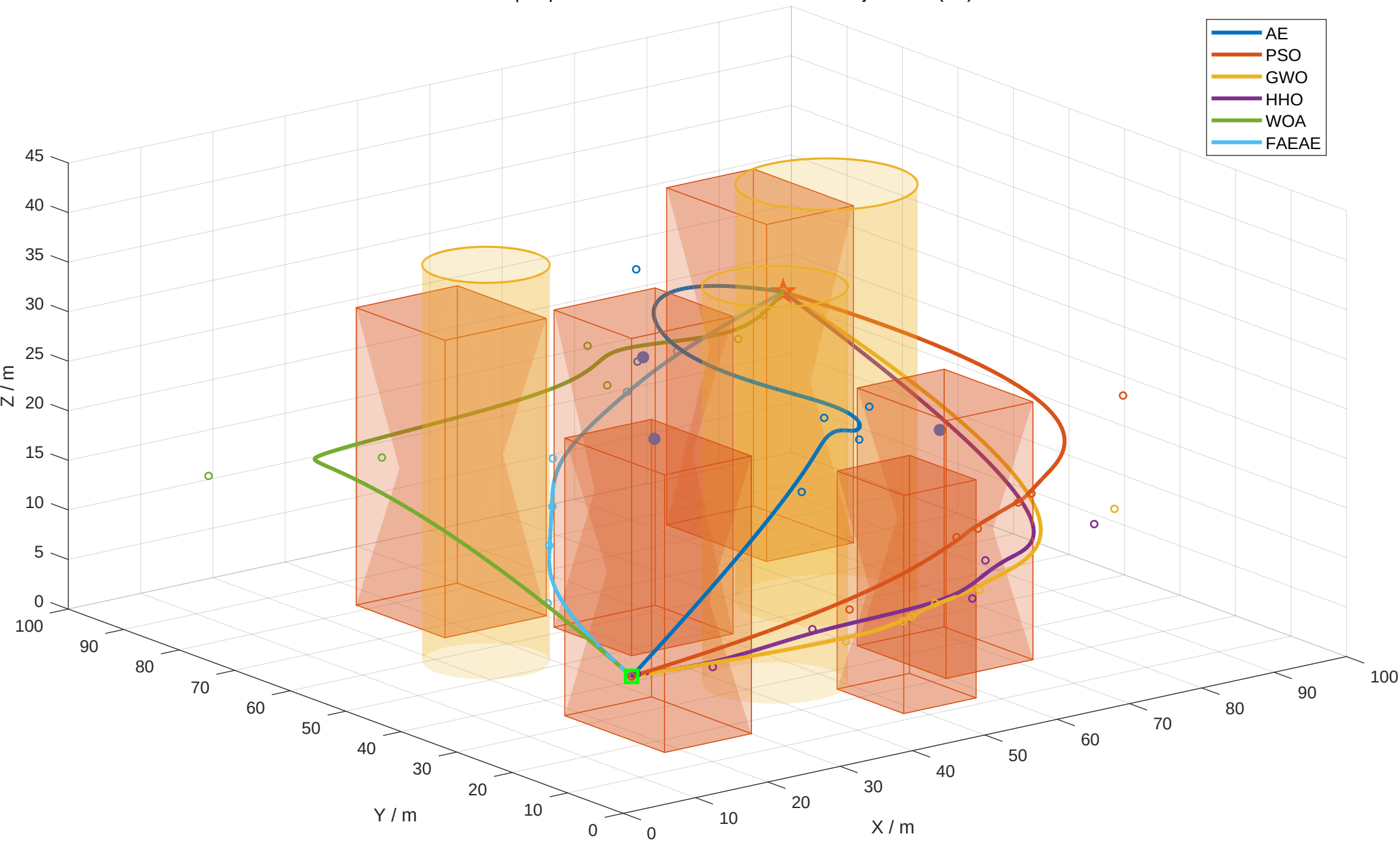
Scene 1 | Representative Low-Altitude Corridor Trajectories (3D)
