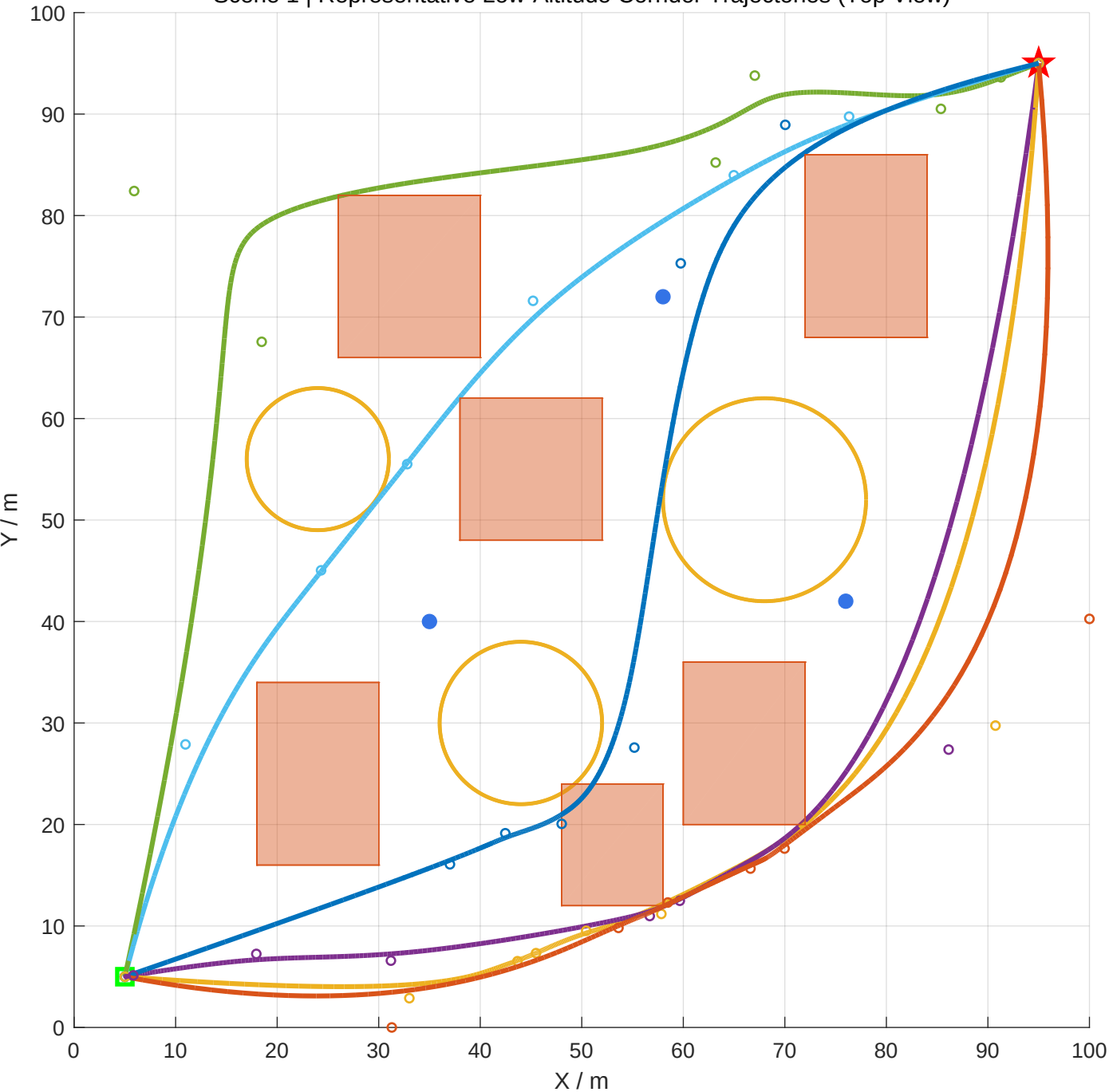
Scene 1 | Representative Low-Altitude Corridor Trajectories (Top View)
