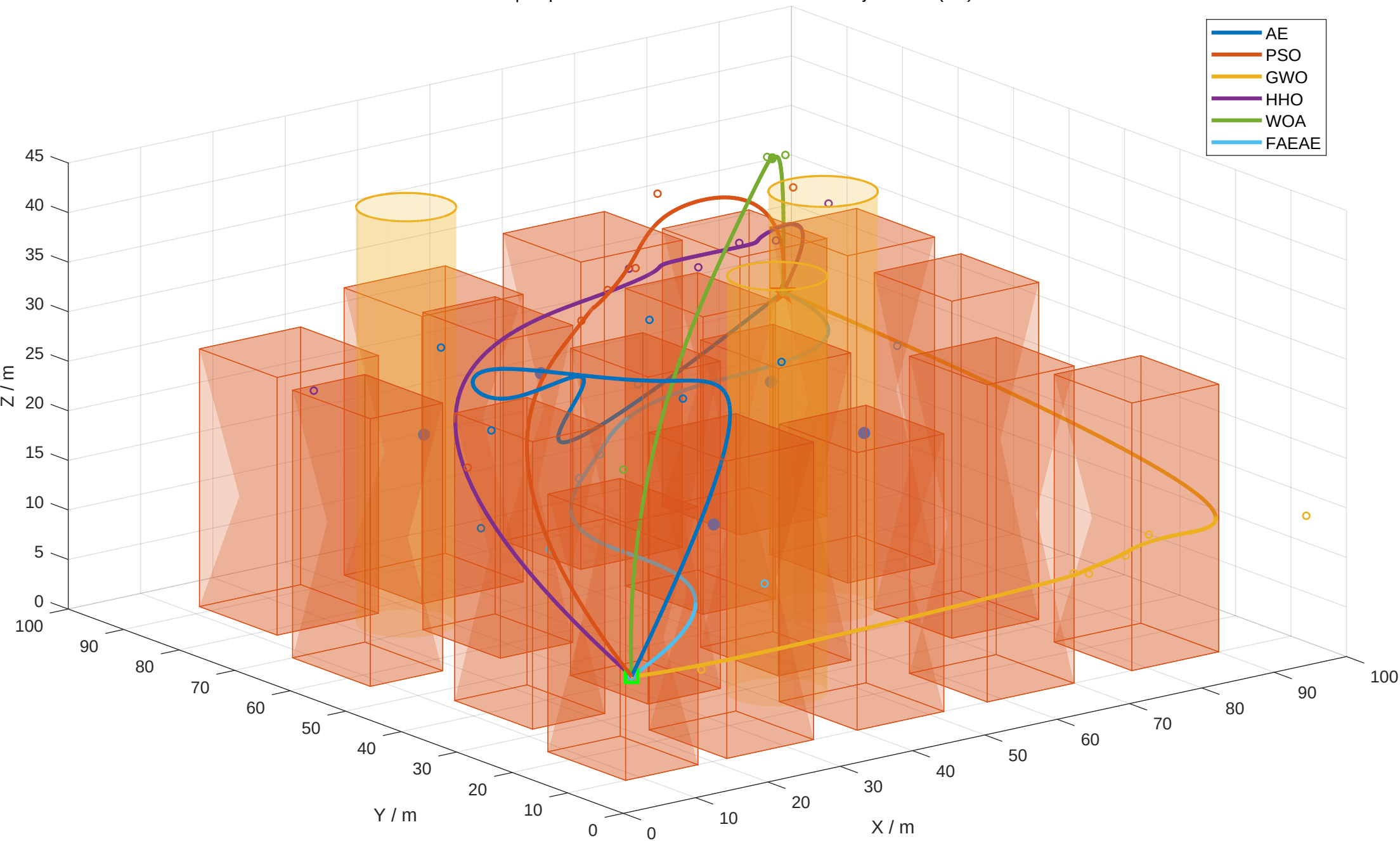
Scene 3 | Representative Low-Altitude Corridor Trajectories (3D)
