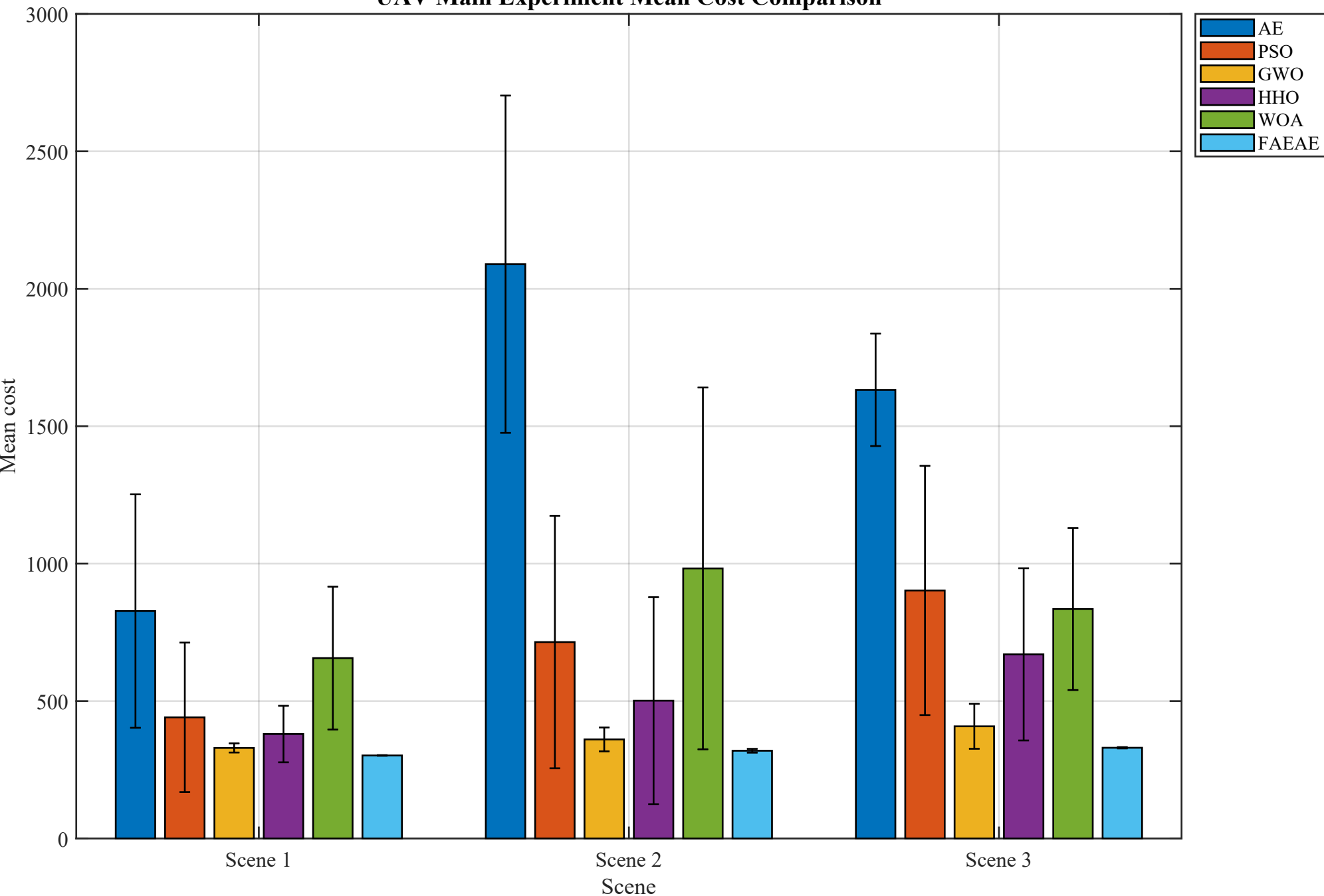
UAV Main Experiment Mean Cost Comparison
