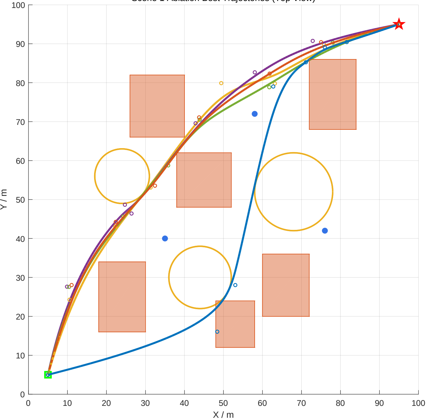
Scene 1 Ablation Best Trajectories (Top View)
