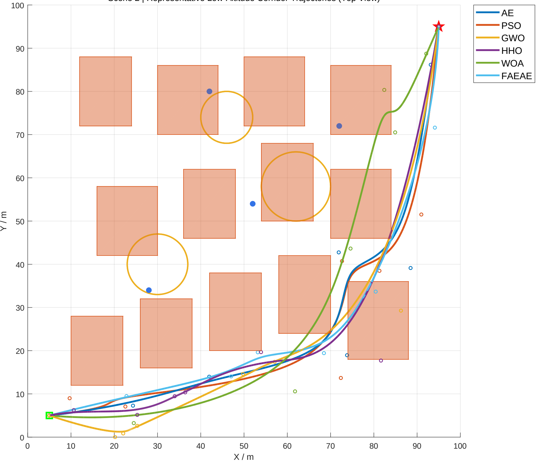
Scene 2 | Representative Low-Altitude Corridor Trajectories (Top View)
