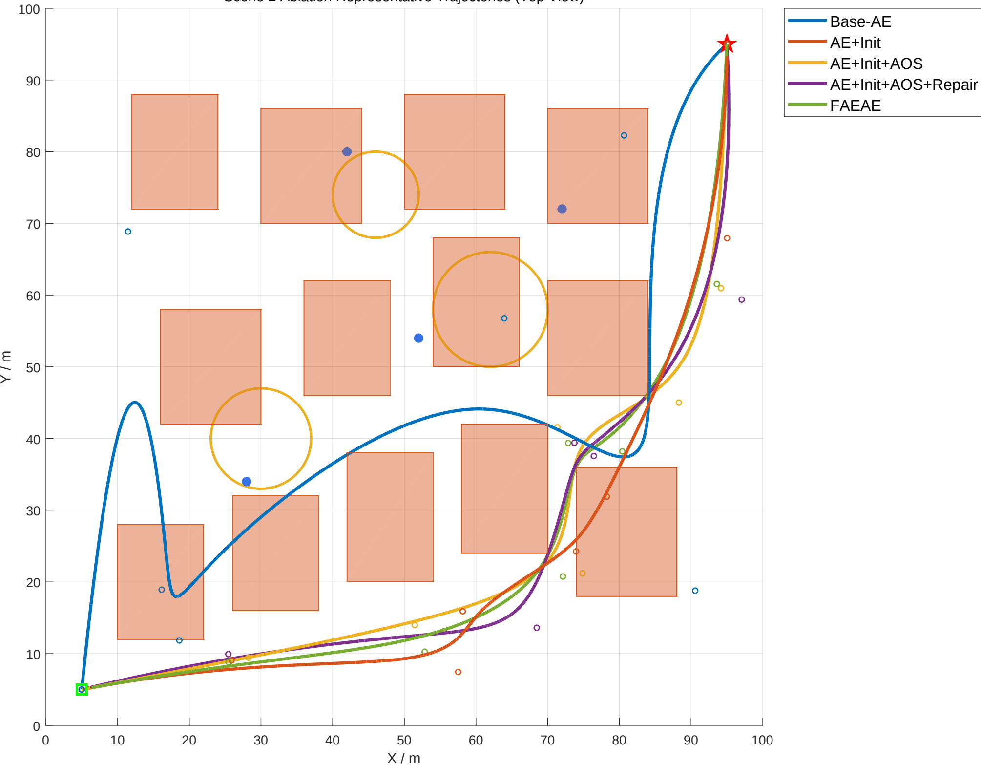
Scene 2 Ablation Representative Trajectories (Top View)
