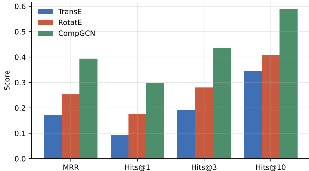
FB15k-237
