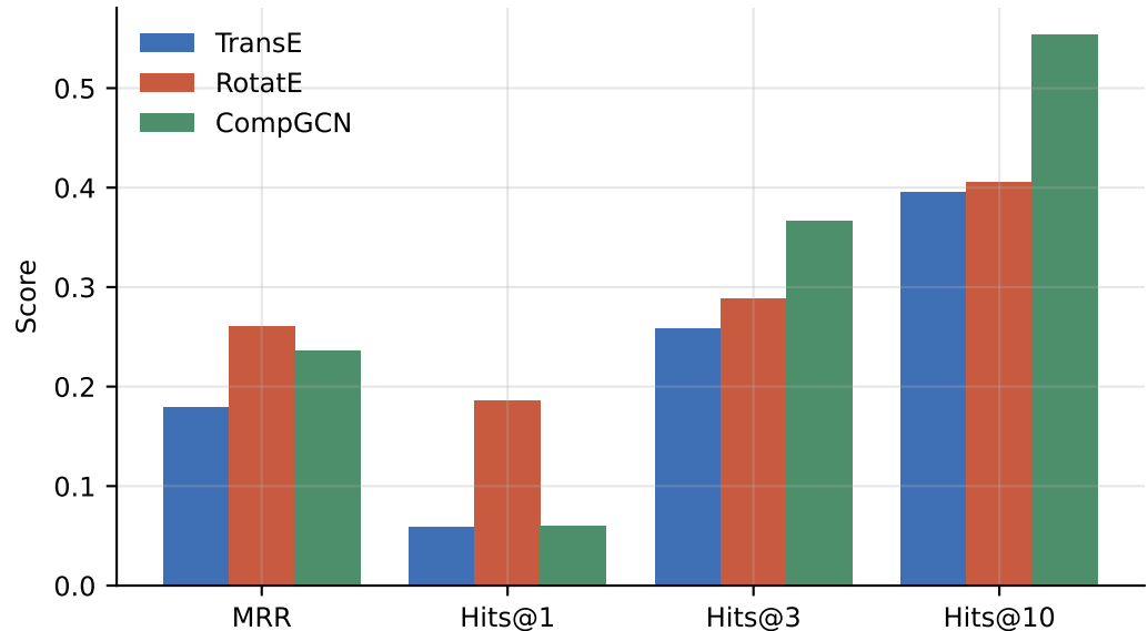
WN18RR
