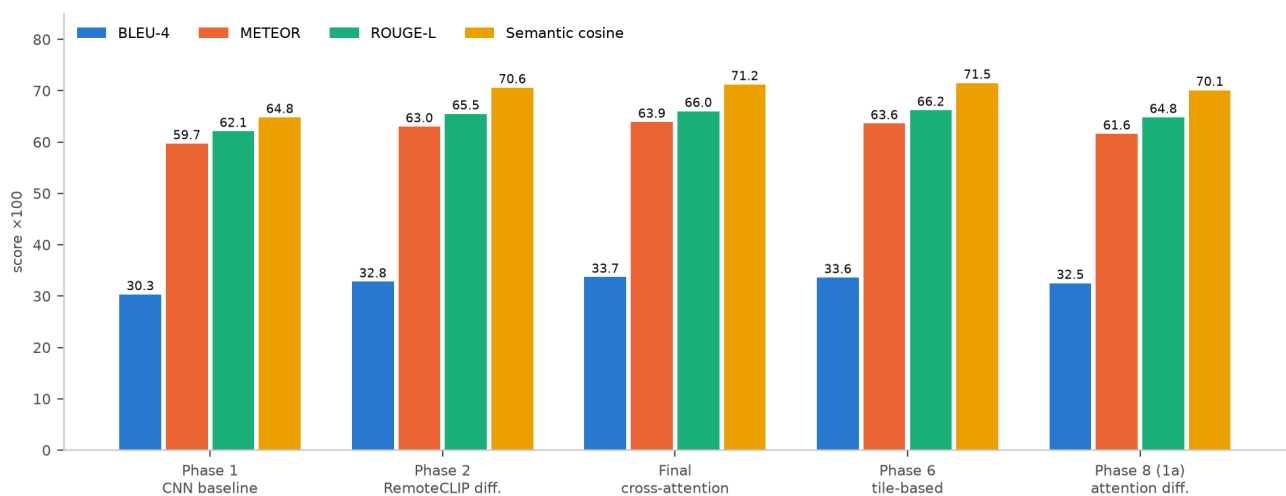
Figure 1. LEVIR-CC test scores per model (Evidence E-A1).
