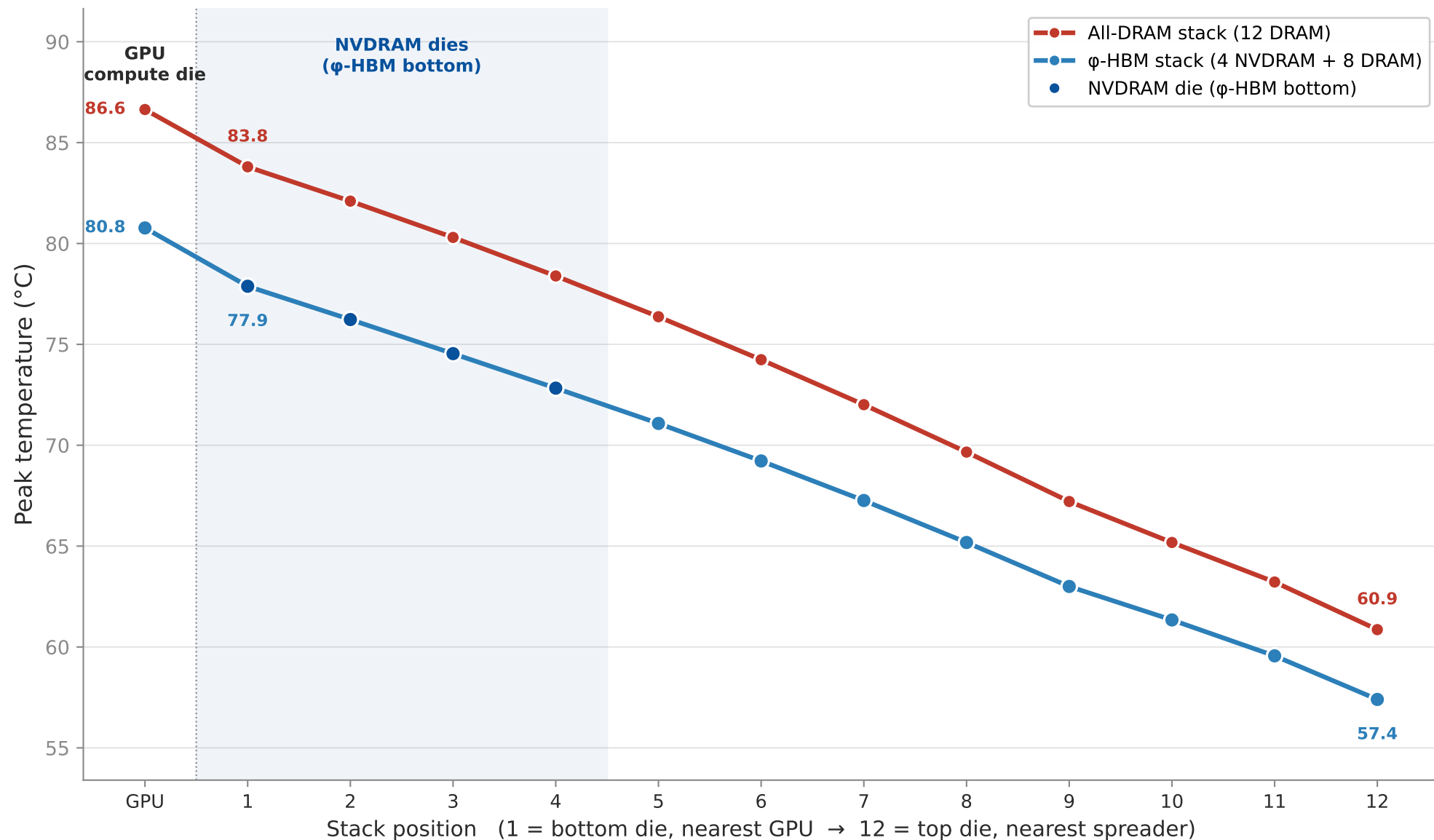
Layerwise stack temperature after thermal-silicon optimization — all-DRAM vs \phi -HBM (30 × 22 mm) Per-die peak under the stacks, active read/write ( \alpha_w=0.24 , 4.4 TB/s/stack, 70/90 fJ/bit)
