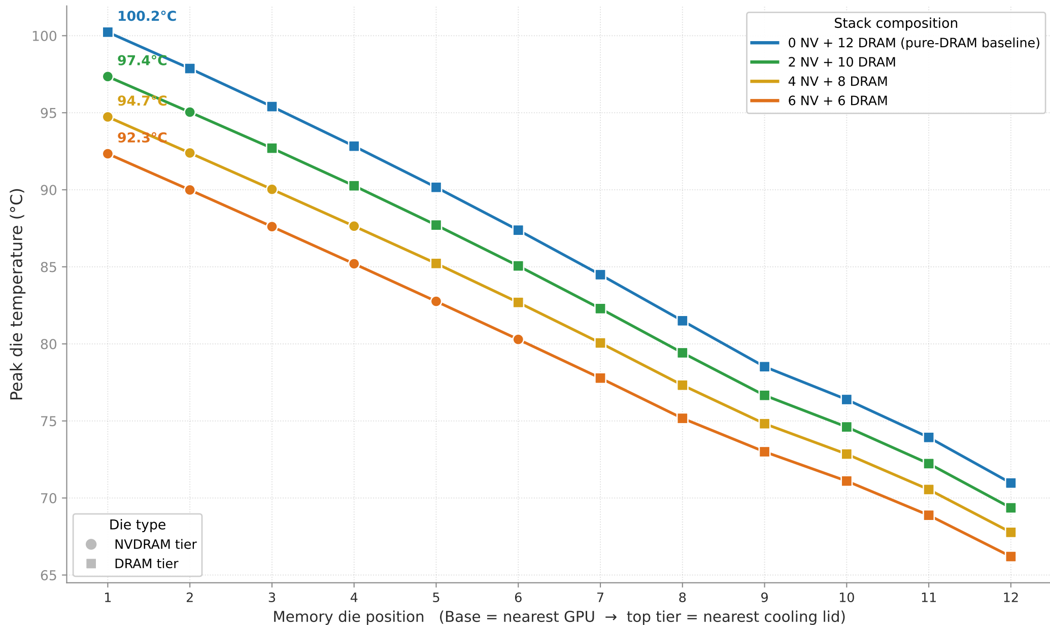
Peak temperature of each memory die up the 3D stack NVDRAM (bottom) + DRAM (top) — varying stack composition (STCO endpoint, no freq scaling)
