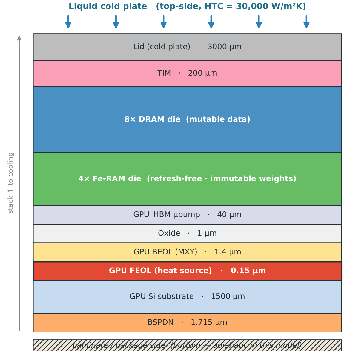
(b) Cross-section (fully STCO-optimized \phi -HBM)
