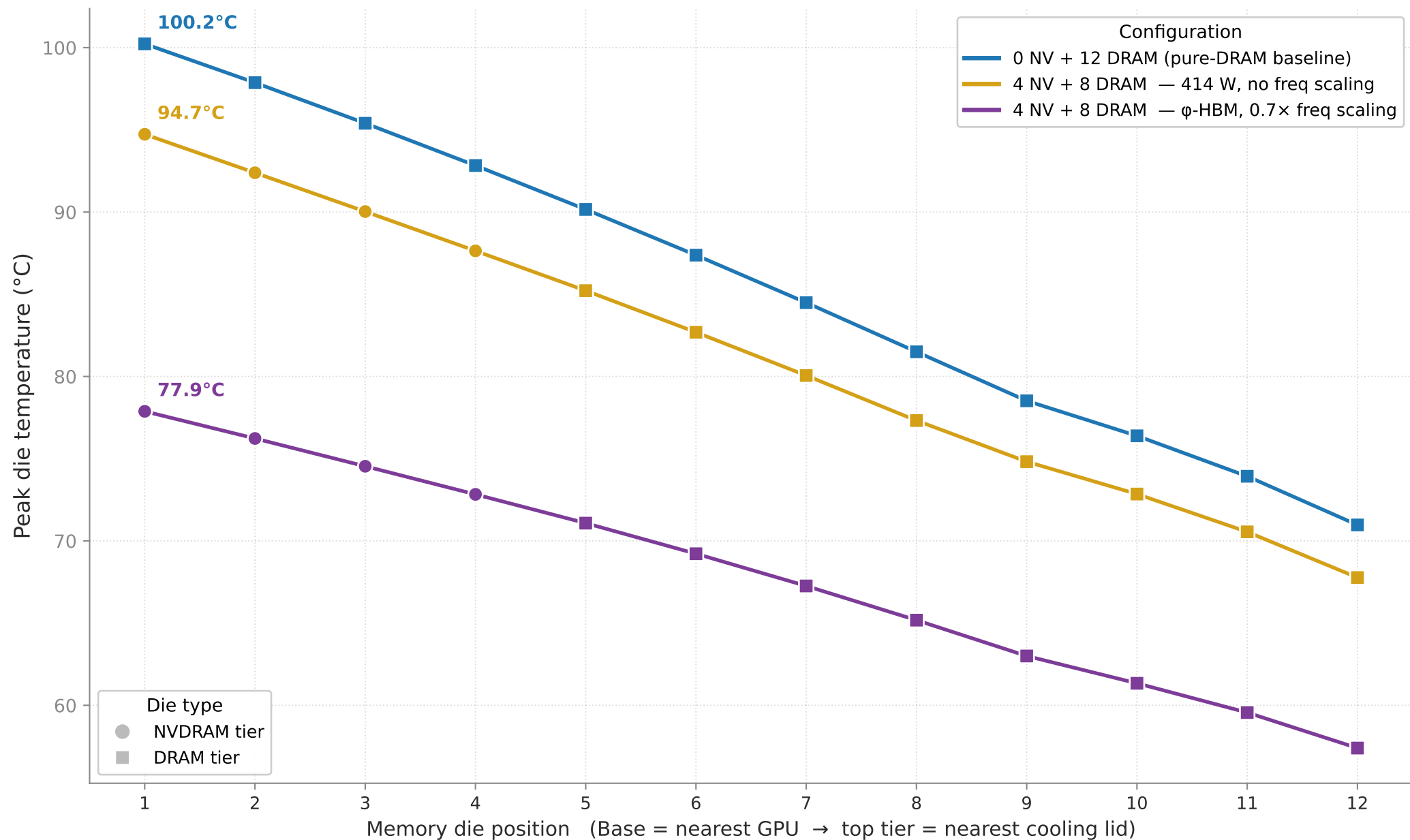
Peak temperature of each memory die up the 3D stack 4 NVDRAM + 8 DRAM: effect of GPU frequency scaling (vs pure-DRAM baseline)
