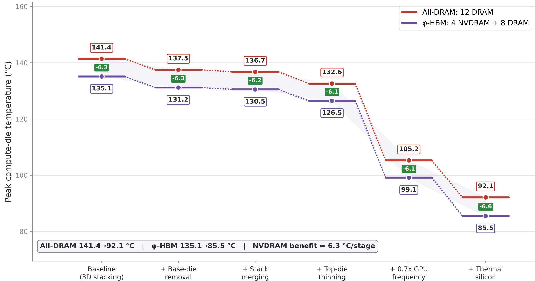
STCO Thermal Waterfall — \phi -HBM vs all-DRAM calibrated to the reference baseline (all-DRAM 3D = 141.4 °C \approx reference 141.7 °C); green = NVDRAM benefit per stage
