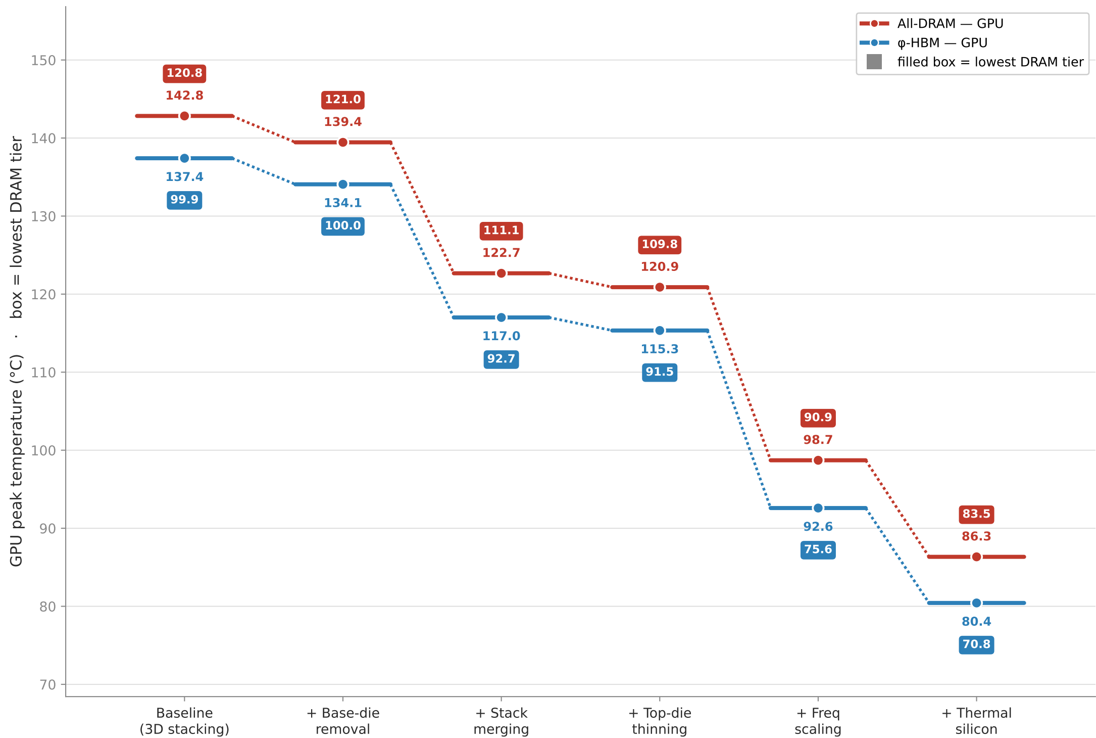
STCO Thermal Waterfall — \phi -HBM vs all-DRAM (30 × 22 mm) GPU compute-die peak (step lines); lowest DRAM tier in the filled box by each GPU number
