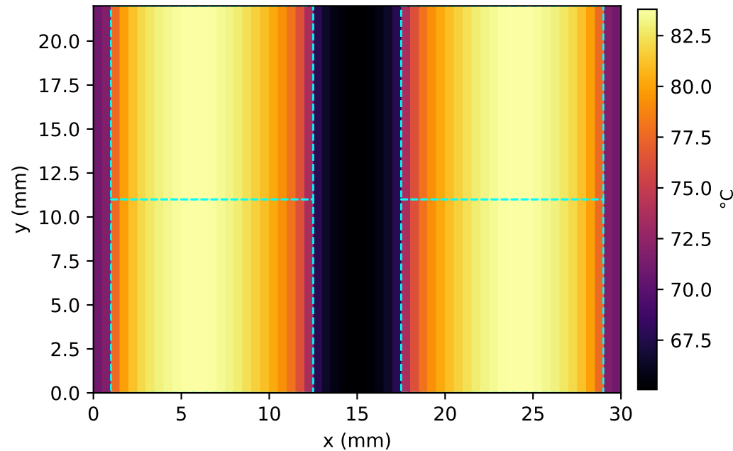
Bottom-most DRAM tier (layer 8) peak 83.8 °C (min 65.1)
