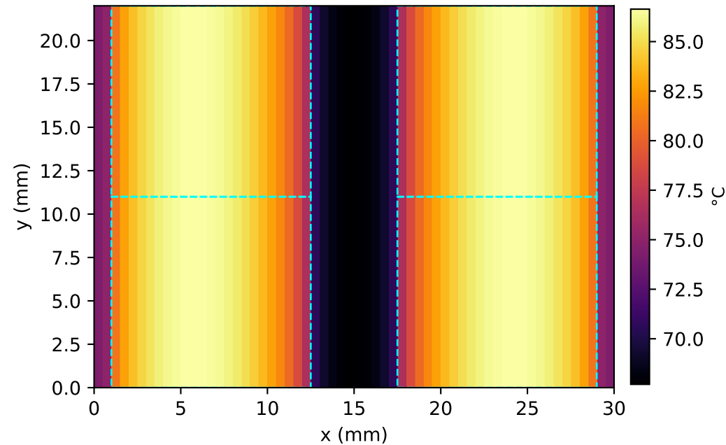
GPU compute die (layer 2) peak 86.6 °C (min 67.7)
