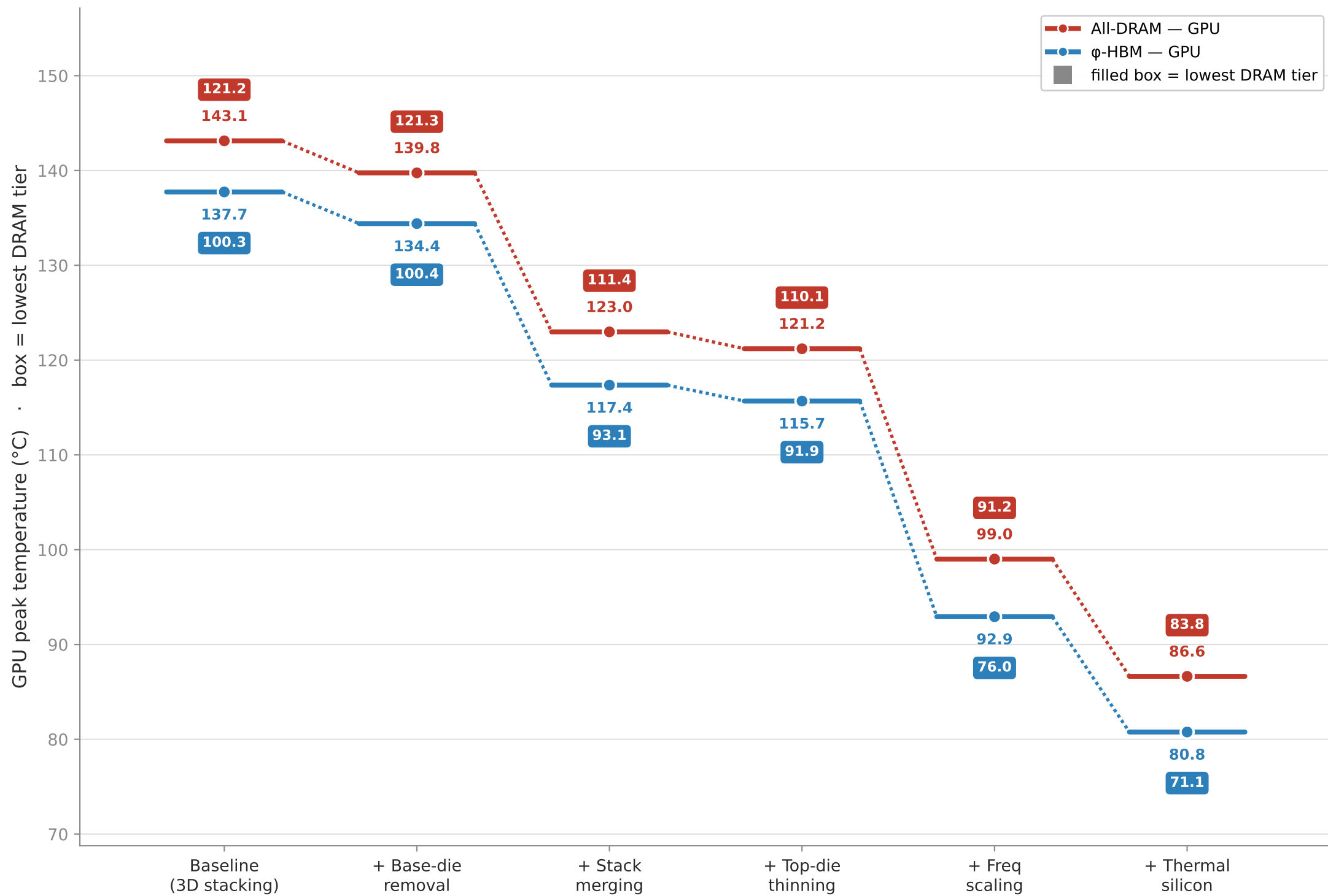
STCO Thermal Waterfall — \phi -HBM vs all-DRAM (30 × 22 mm), active read/write GPU compute-die peak (step lines); lowest DRAM tier in the filled box by each GPU number
