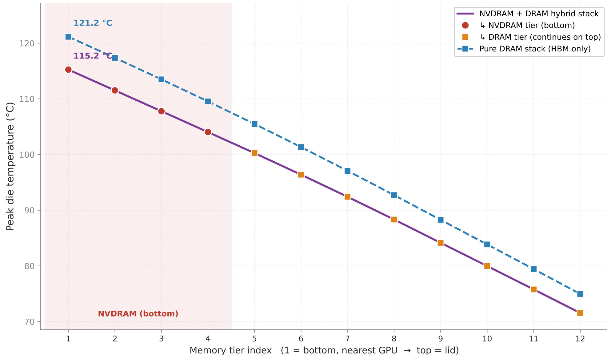
Layerwise stack temperature — 3D-stacking baseline (no optimizations) all-DRAM vs \phi -HBM (30 × 22 mm); per-die peak under the stacks, active read/write ( \alpha_w=0.24 , 4.4 TB/s/stack, 70/90 fJ/bit)
