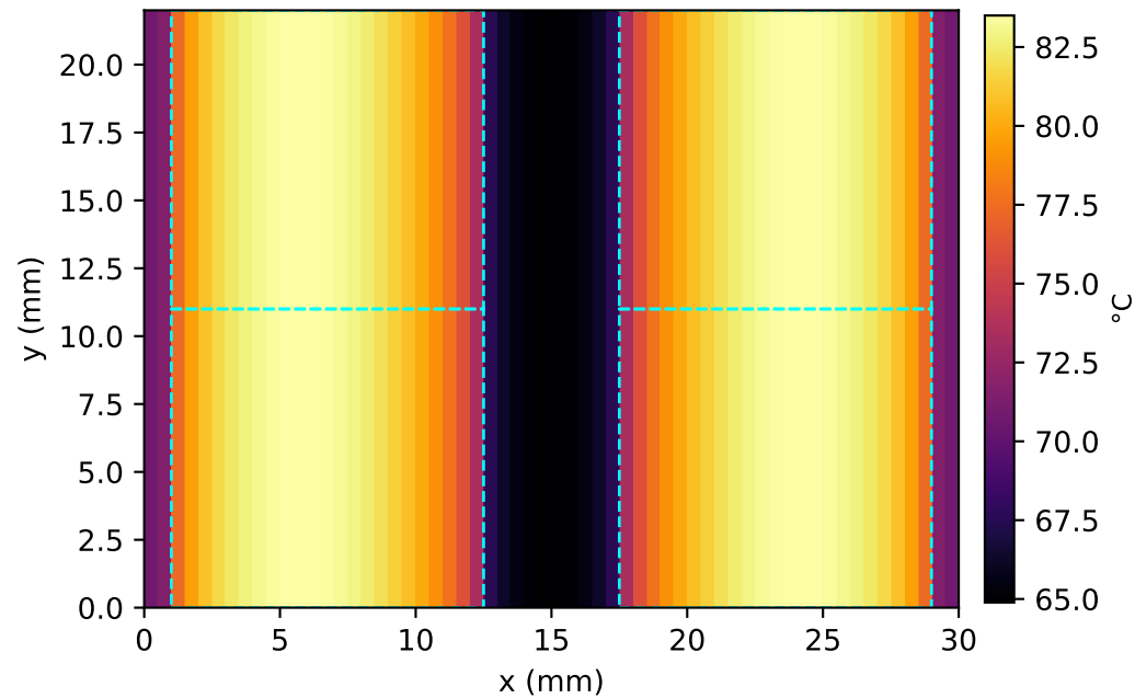
Bottom-most DRAM tier (layer 8) peak 83.5 °C (min 64.9)
