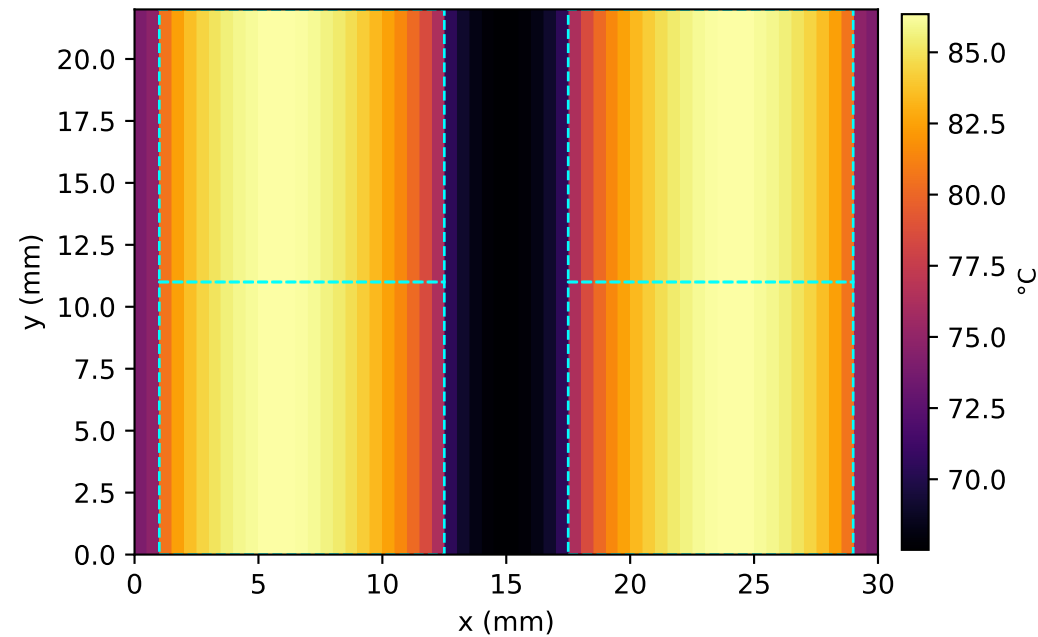
GPU compute die (layer 2) peak 86.3 °C (min 67.5)
