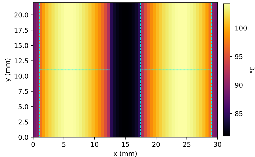
GPU compute die (layer 2) peak 104.2 °C (min 81.1)
