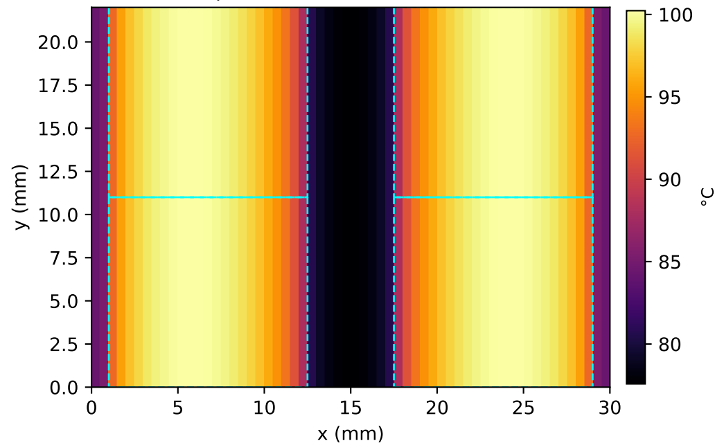
Bottom-most DRAM tier (layer 8) peak 100.2 °C (min 77.6)
