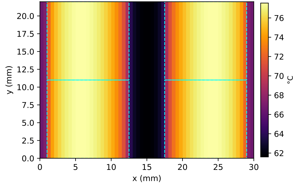
Lowest NVDRAM tier (layer 8) peak 77.5 °C (min 61.6)
