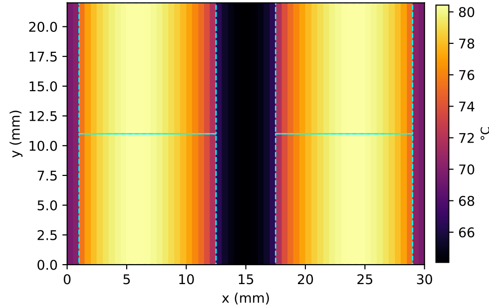
GPU compute die (layer 2) peak 80.4 °C (min 64.1)
