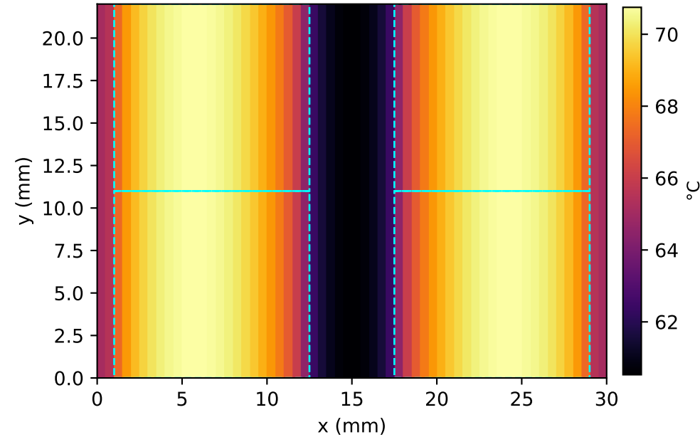
Lowest DRAM tier (layer 20) peak 70.8 °C (min 60.5)
