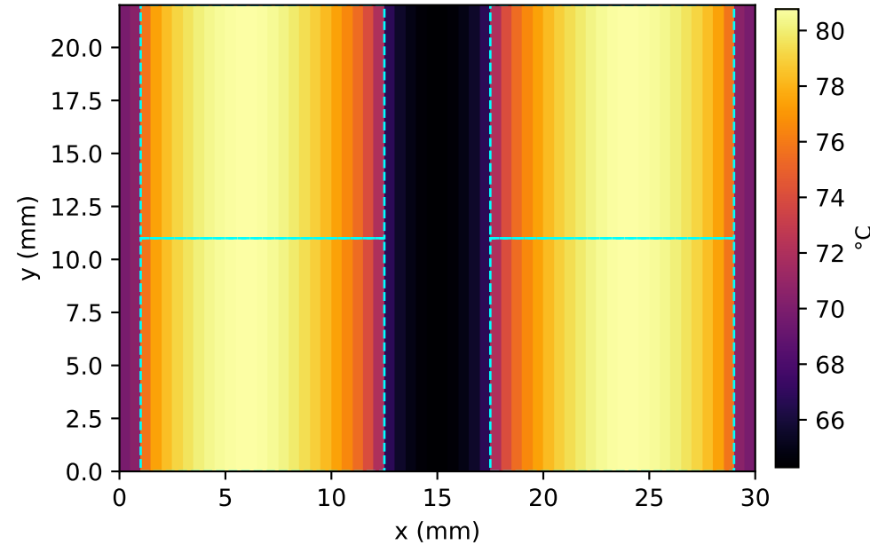
GPU compute die (layer 2) peak 80.8 °C (min 64.3)
