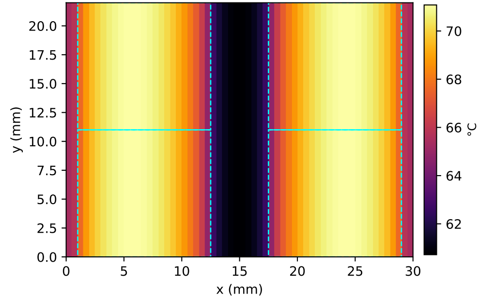
Lowest DRAM tier (layer 20) peak 71.1 °C (min 60.7)
