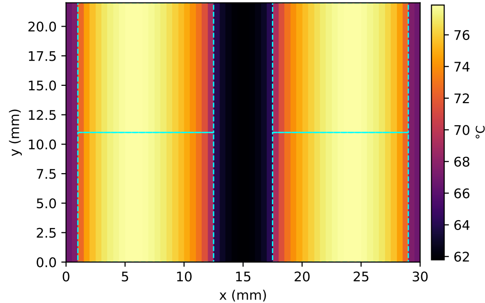
Lowest NVDRAM tier (layer 8) peak 77.9 °C (min 61.8)
