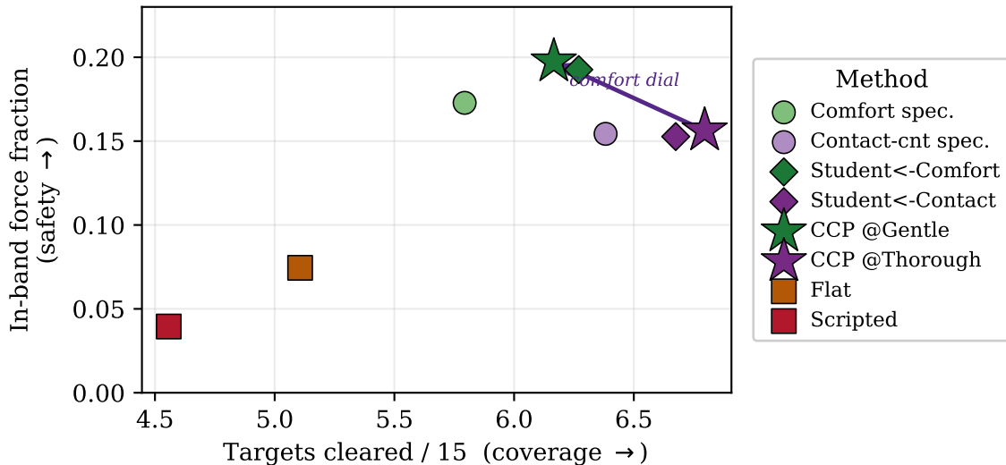
One policy, two behaviours: the comfort dial spans the safety \leftrightarrow coverage frontier; baselines are strictly dominated
