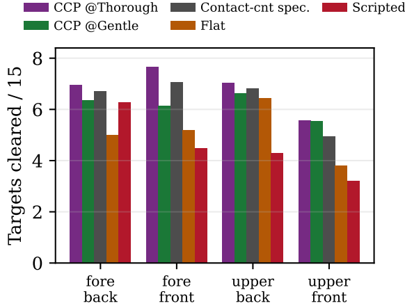
Fig. 3. Targets cleared per region. CCP (both settings) exceeds the flat and scripted baselines in every region; the residual gap on back regions is a physical reachability limit (Sec. VII), not a policy failure.
